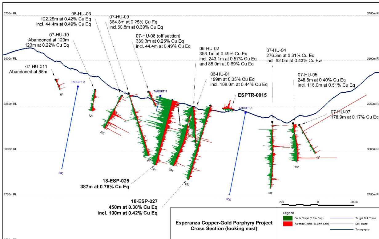
Figure 1: North South cross section showing complete results from 18-ESP-025 and 18-ESP-027, surface road cut sampling, and two of the four priority drill targets.
