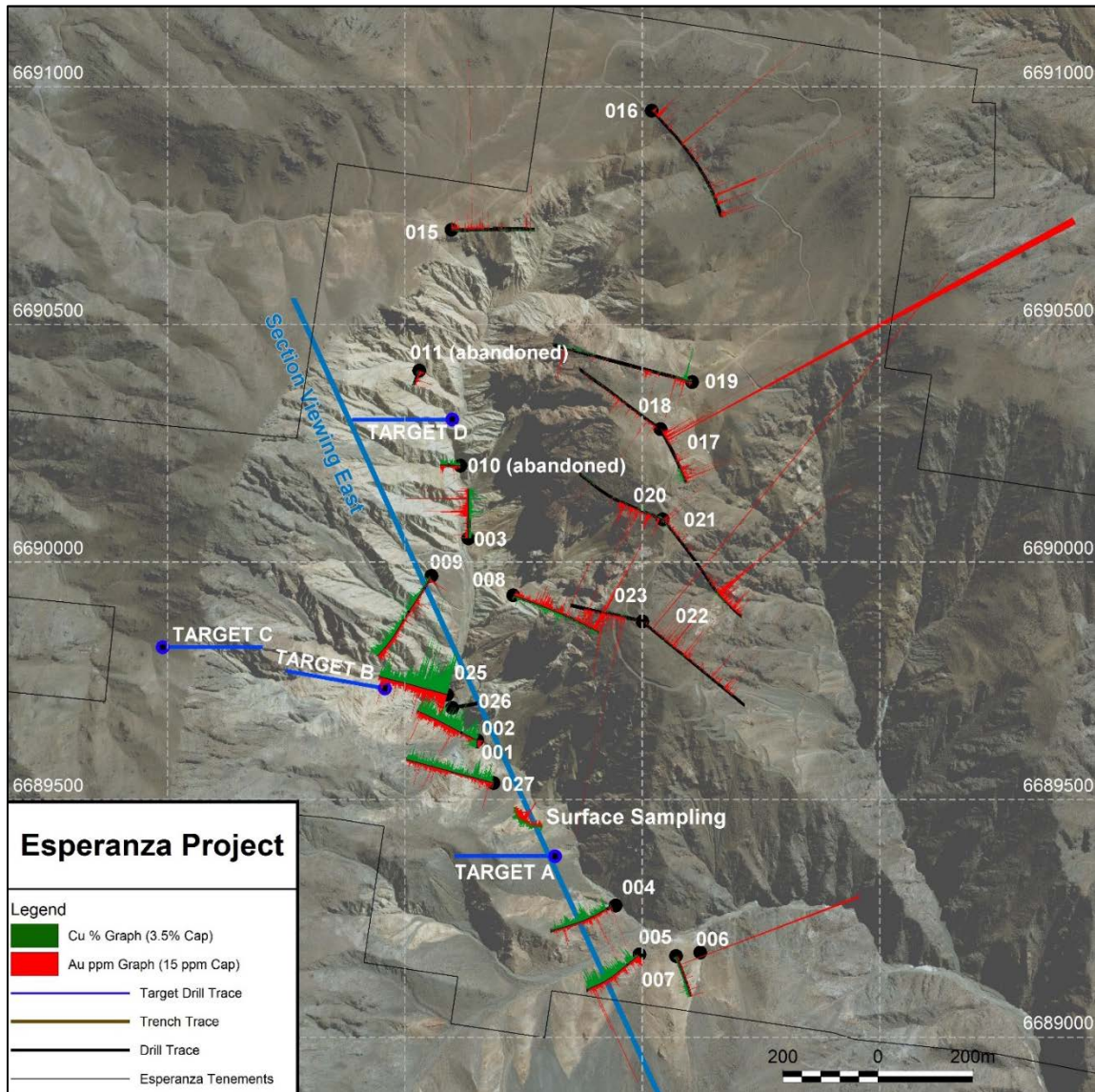
Figure 2: Map showing all drill holes completed on the property as well as 2018 surface sampling.
