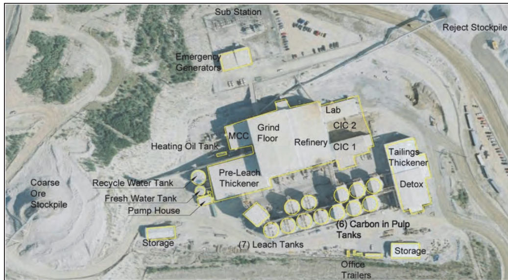
Figure 17-2: Fort Knox Mill Complex Site Plan.
