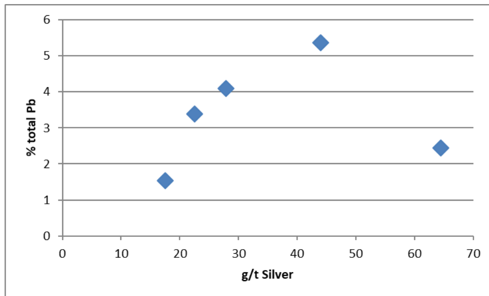
Figure 13-1 Lead vs Silver Content 2017 Metallurgical Composites
