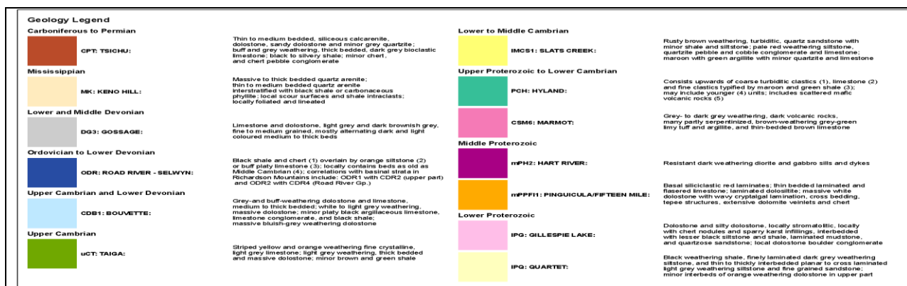
Figure 7-1 Regional Geology
