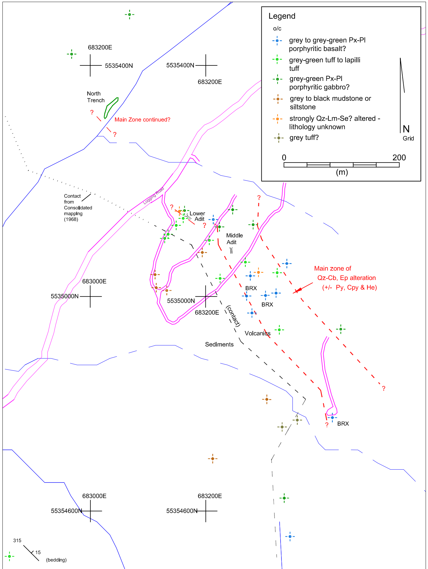
Figure 19: Wen Prospect geology map
