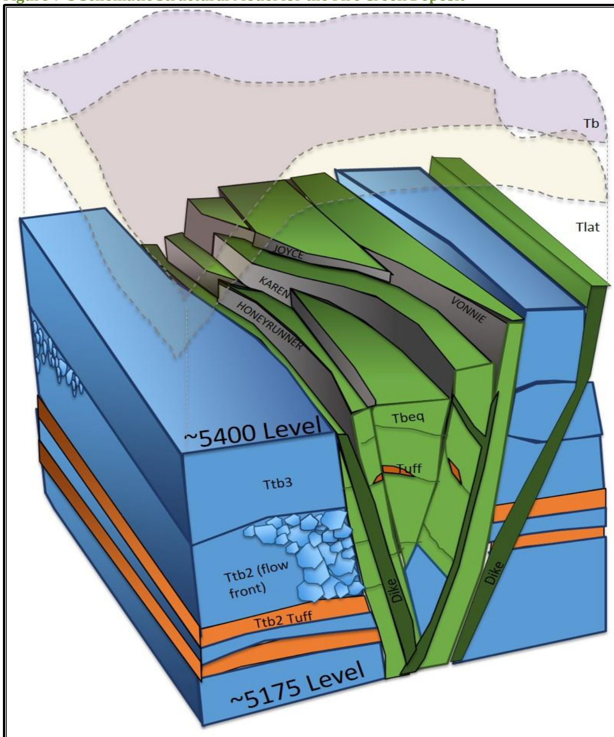
Figure 7-5 Schematic Structural Model for the Fire Creek Deposit
