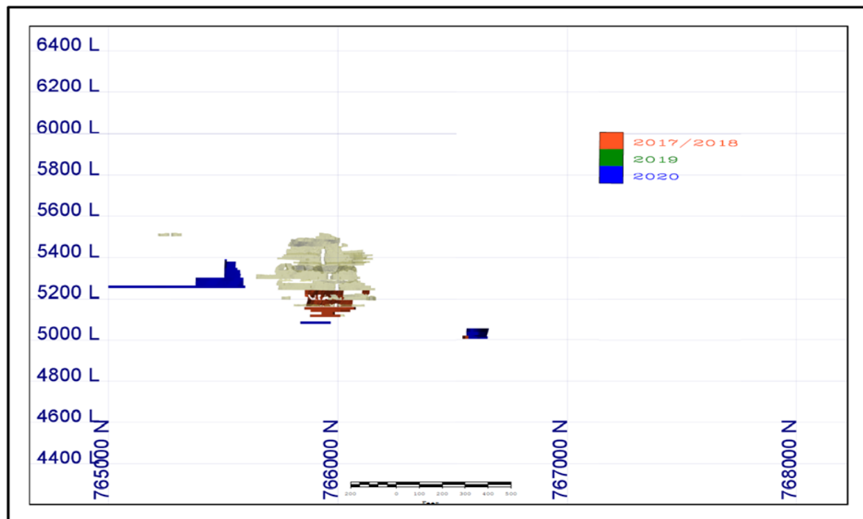
Figure 16-5 Vonnie Vein Long Section Looking West Showing Existing Mine Workings and Reserves Mine Plan
