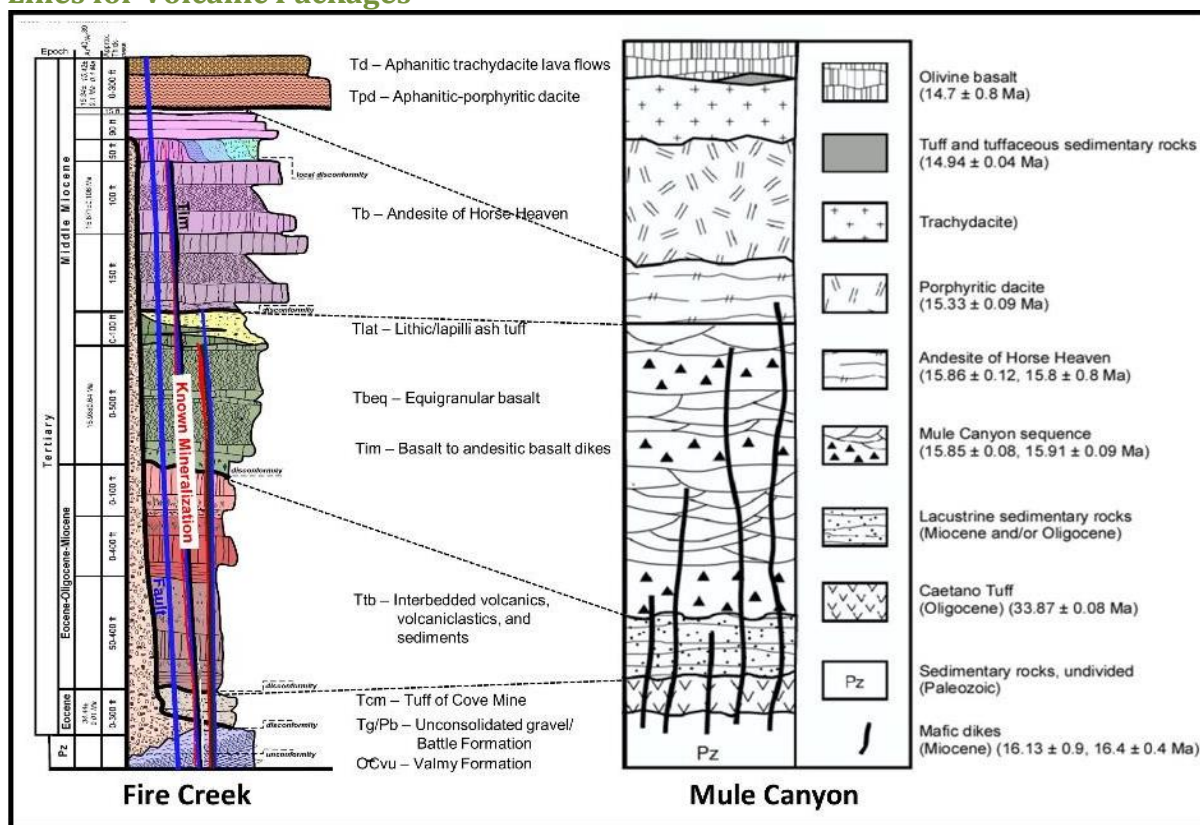
Figure 7-3 Stratigraphic Sections for the Project and the Mule Canyon Mine with Tie Lines for Volcanic Packages
