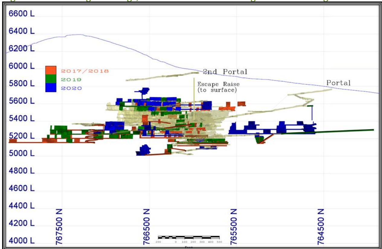
Figure 15-1 Existing Workings, Reserve Excavations Long Section Looking East
