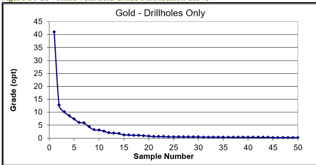
Figure 14-16 Vonnie Vein Gold Grade Distribution Curve
