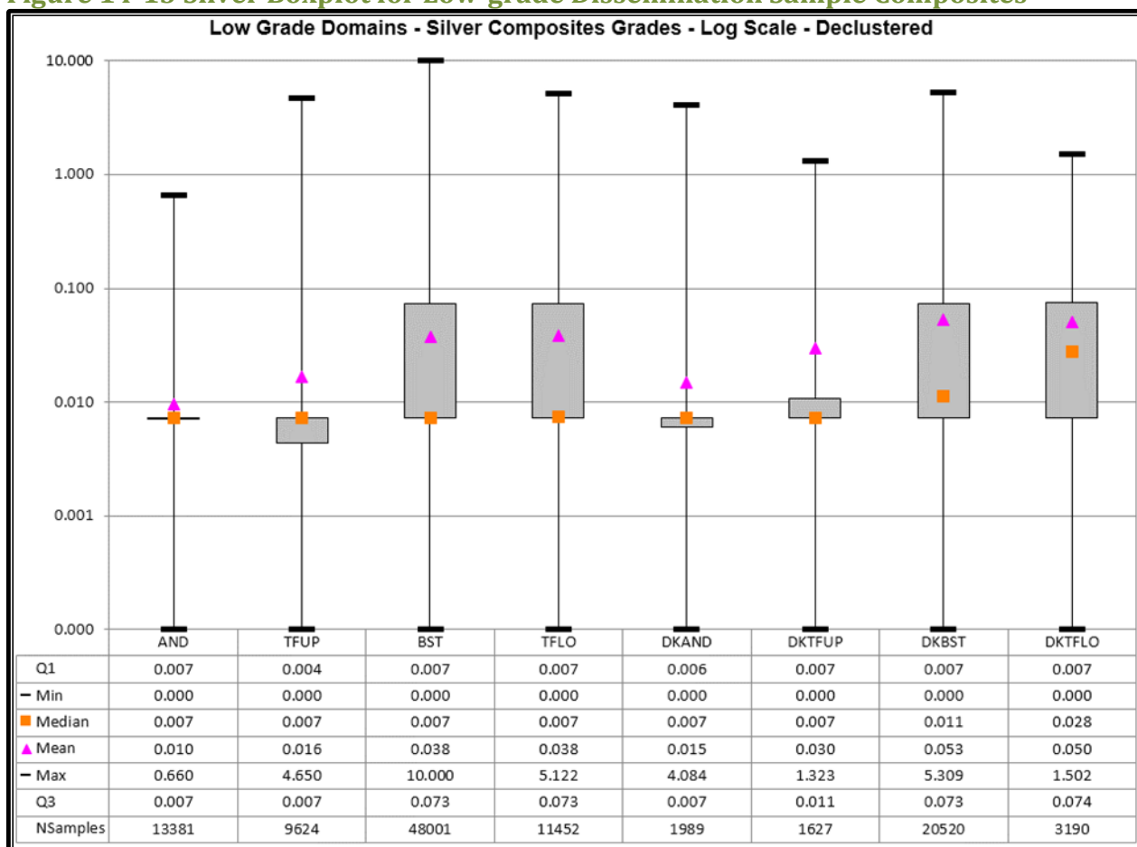
Figure 14-13 Silver Boxplot for Low-grade Dissemination Sample Composites
