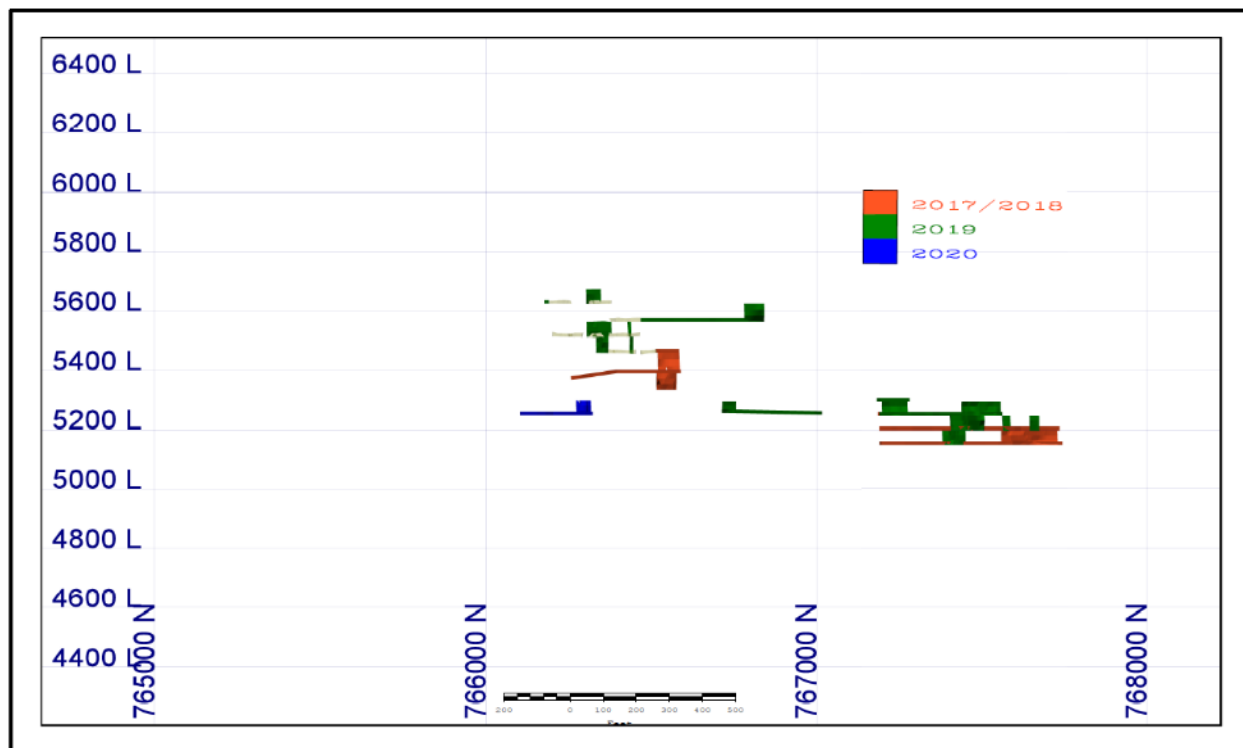
Figure 16-7 Vein 20 Long Section Looking West Showing Existing Mine Workings and Reserves Mine Plan
