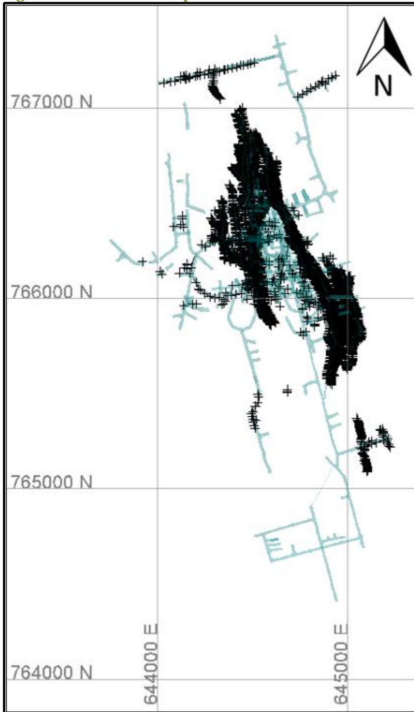
Figure 10-4 Channel Sample Locations
