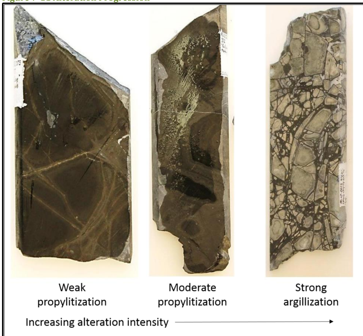
Figure 7-11 Alteration Progression
