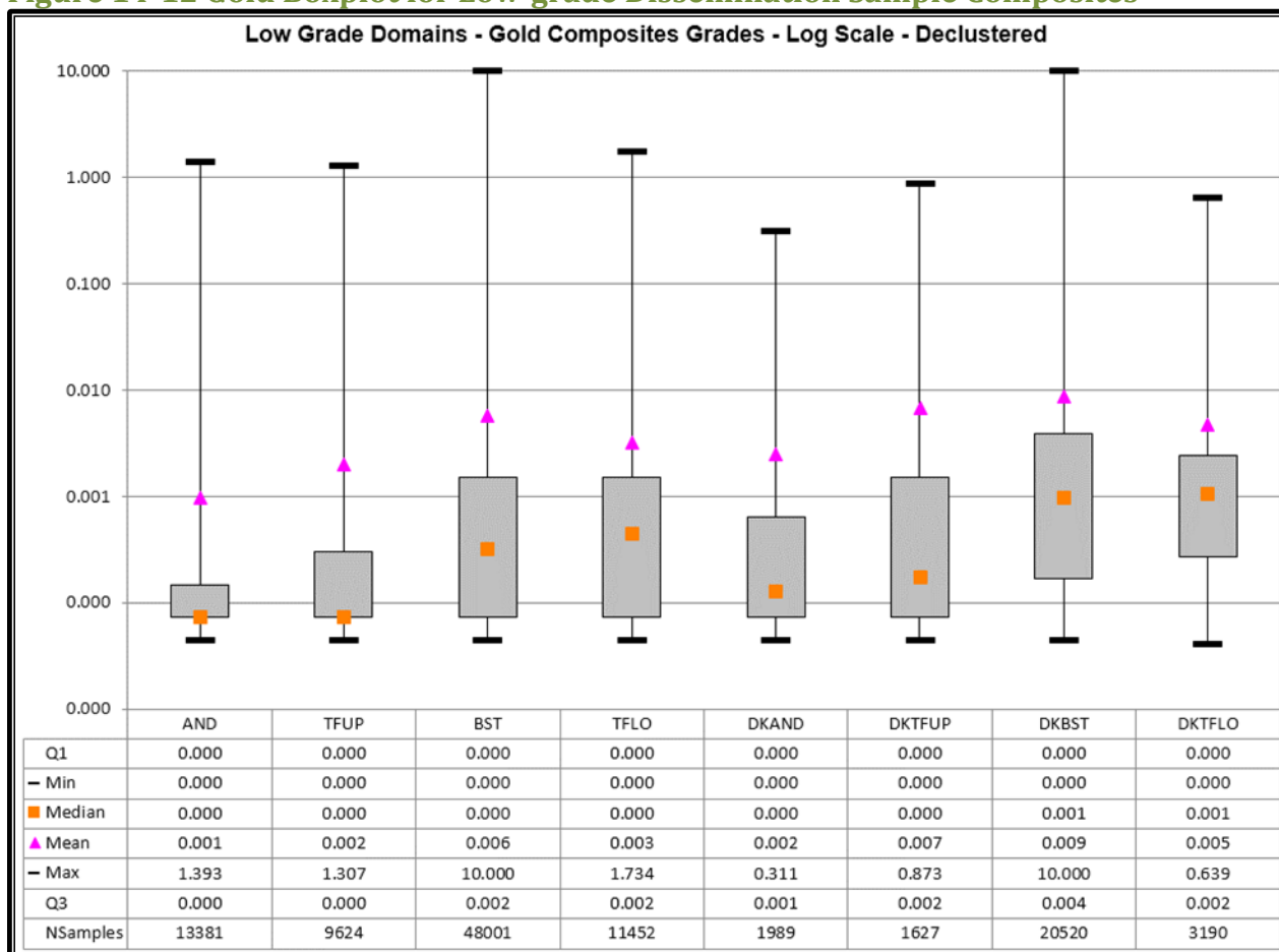
Figure 14-12 Gold Boxplot for Low-grade Dissemination Sample Composites
