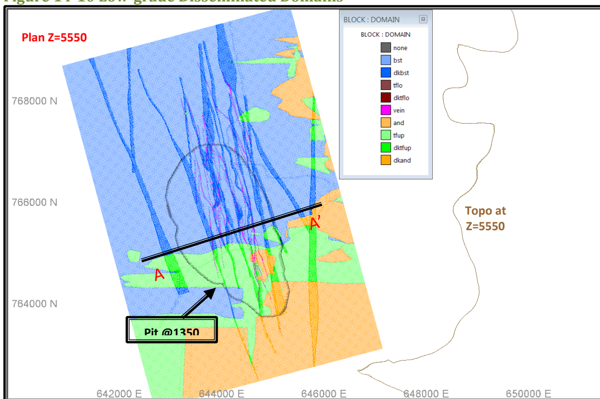
Figure 14-10 Low-grade Disseminated Domains
