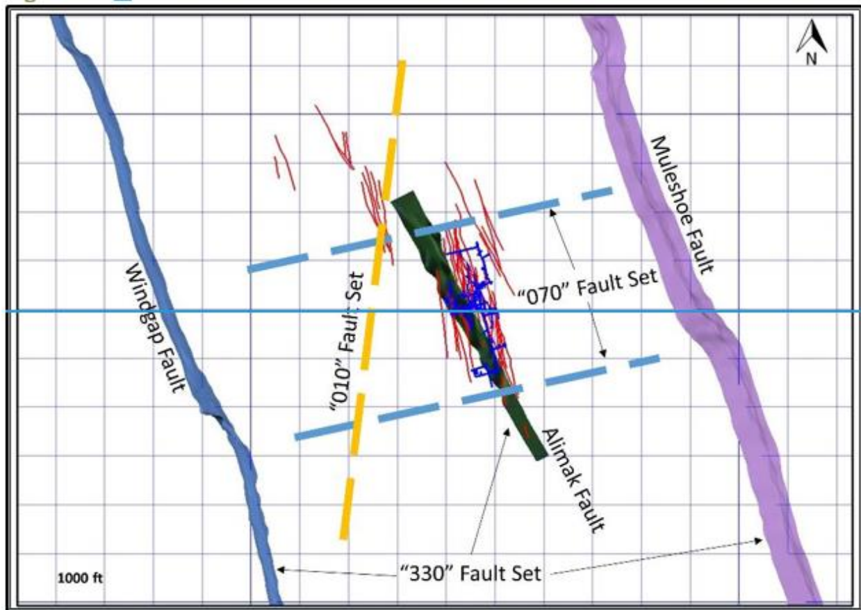
Figure 7-9 Fault Locations
