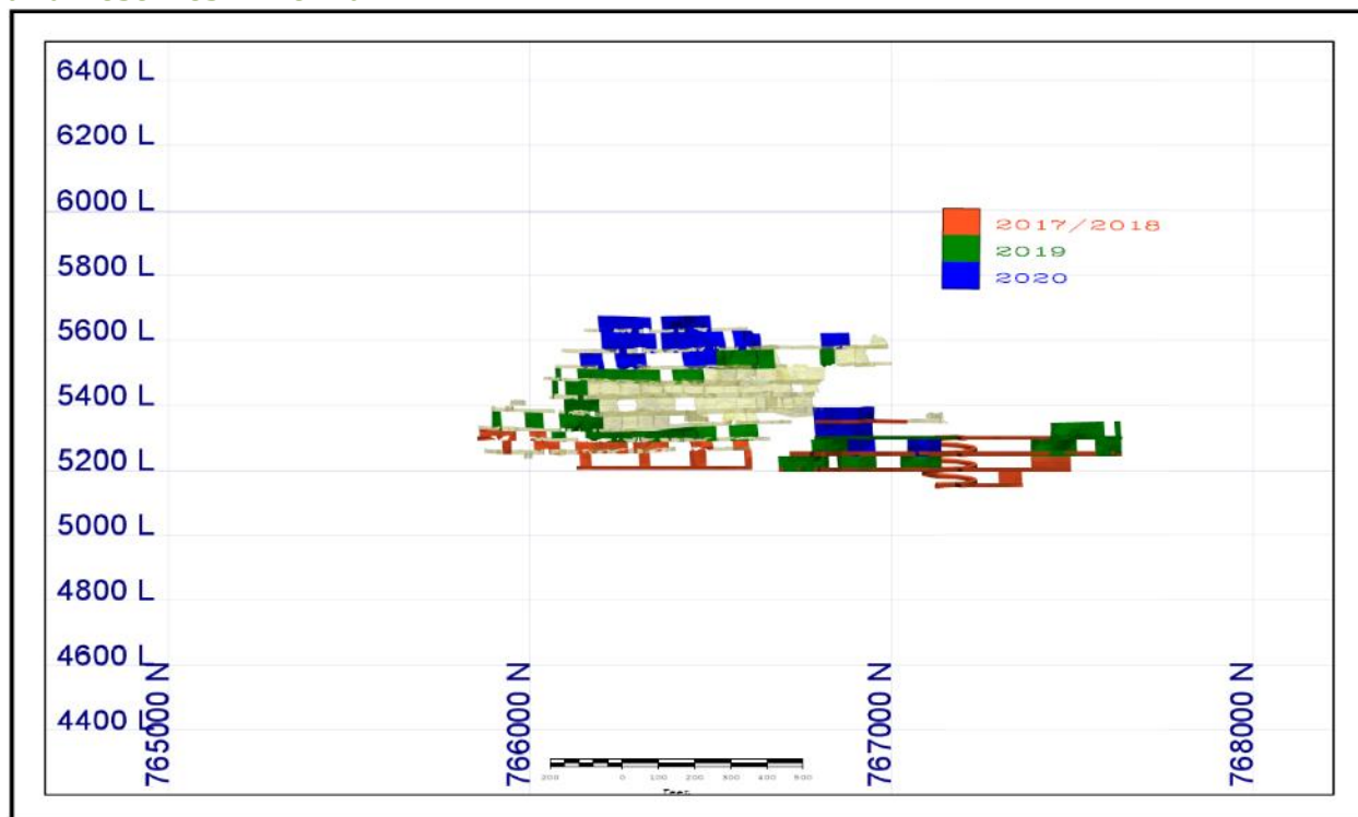
Figure 16-6 Karen Vein Long Section Looking West Showing Existing Mine Workings and Reserves Mine Plan
