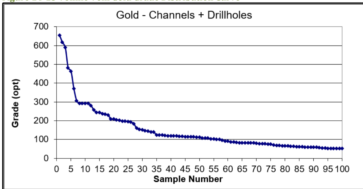
Figure 14-15 Vonnie Vein Gold Grade Distribution Curve
