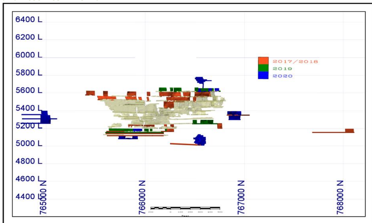
Figure 16-4 Joyce Vein Long Section Looking West Showing Existing Mine Workings and Reserves Mine Plan
