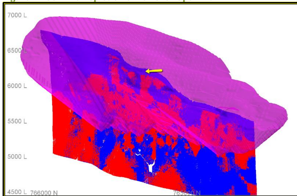
Figure 14-38 Mine Depletion of Veins for Open Pit
