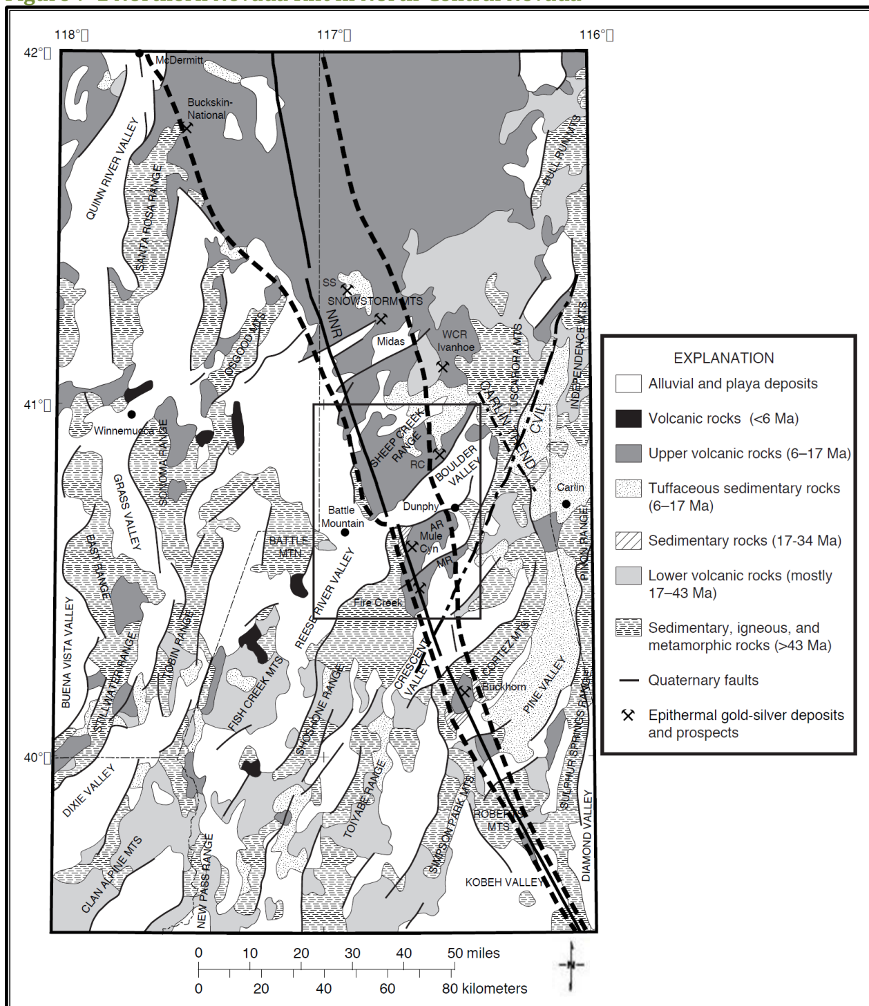
Figure 7-1 Northern Nevada Rift in North-Central Nevada
