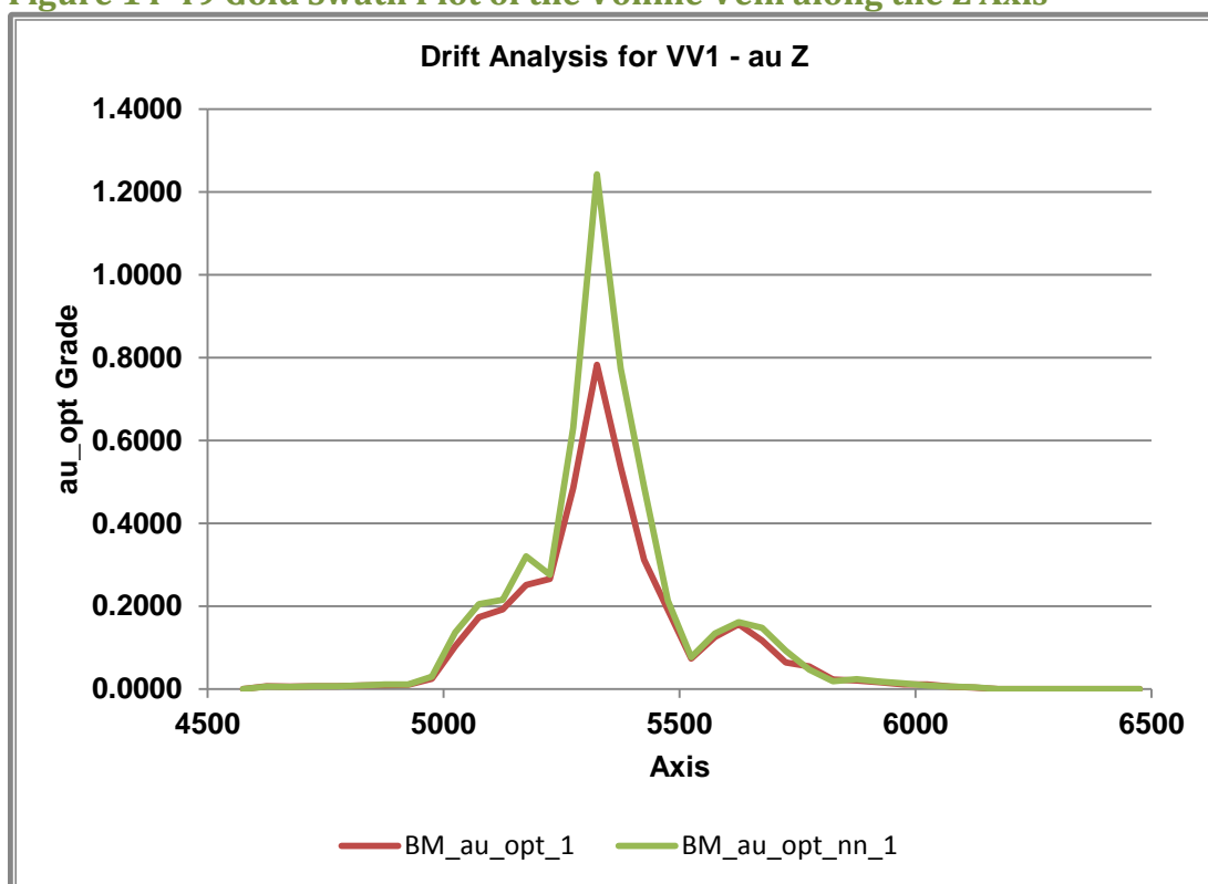
Figure 14-49 Gold Swath Plot of the Vonnies Vein along the Z Axis
