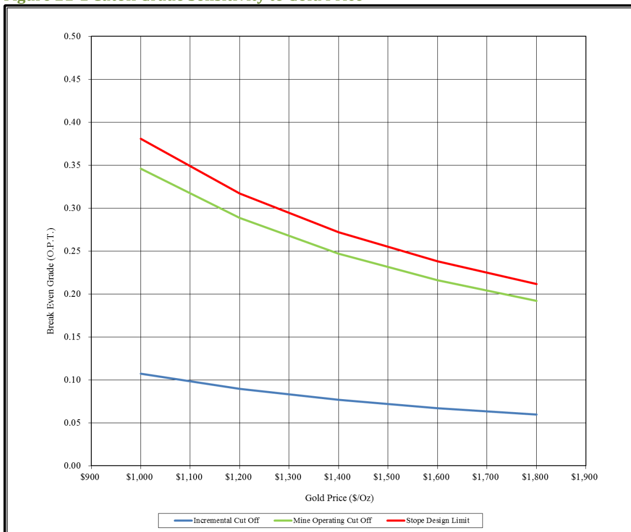
Figure 21-1 Cutoff Grade Sensitivity to Gold Price
