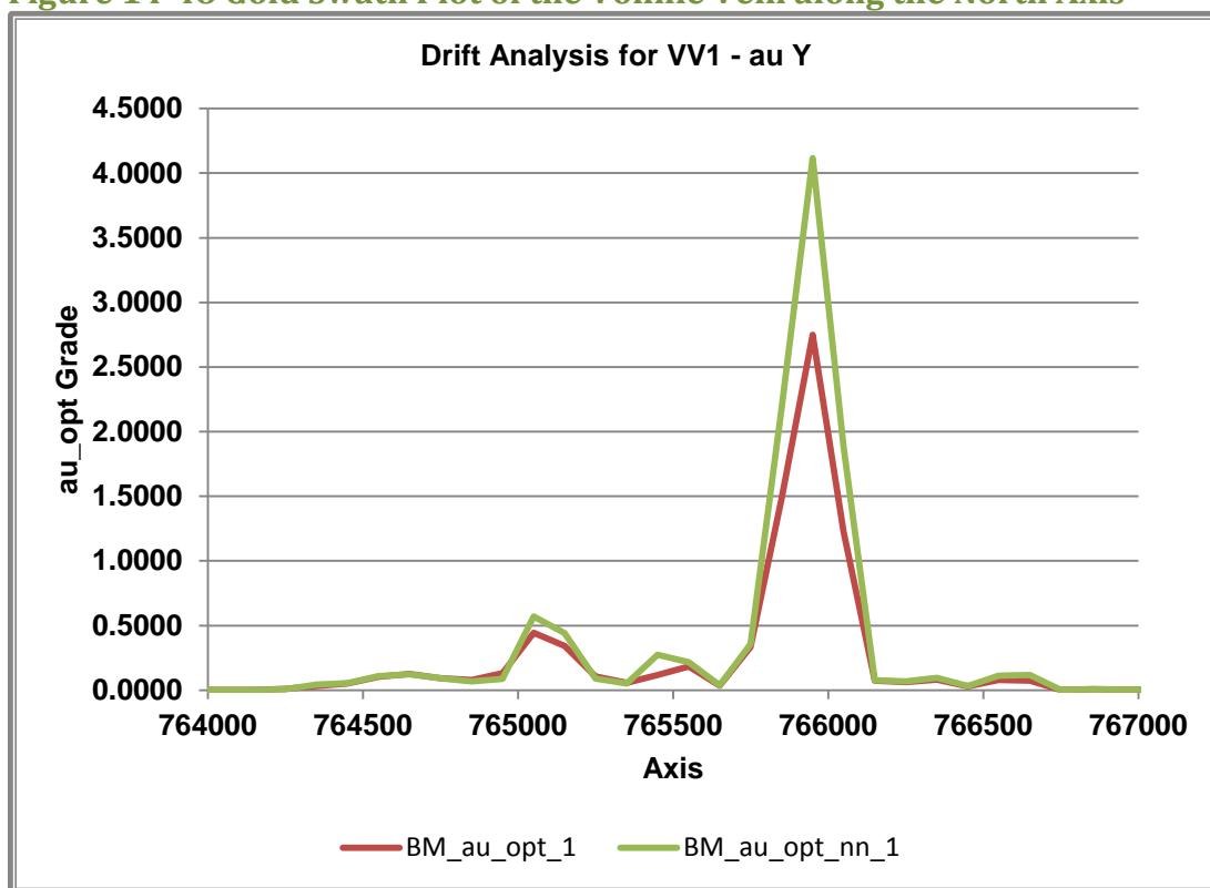
Figure 14-48 Gold Swath Plot of the Vonnies Vein along the North Axis
