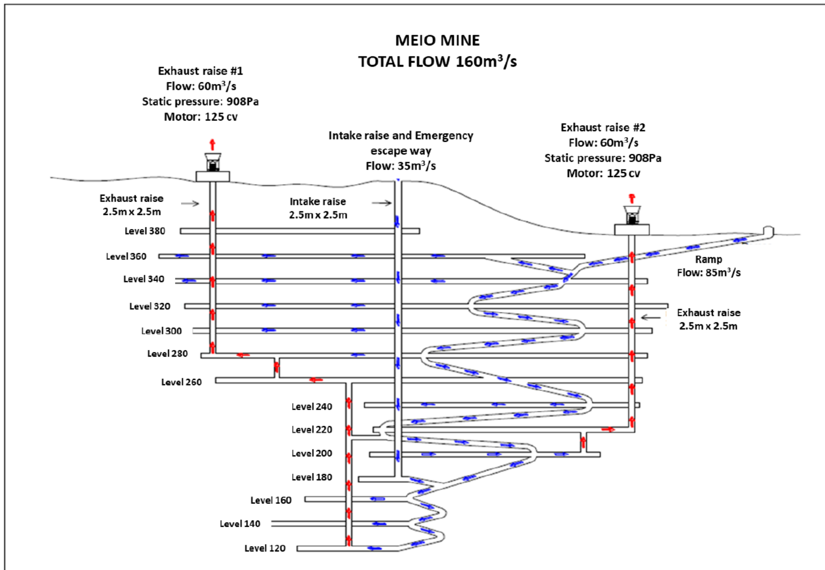
Figure 1.8: Airflow Paths - Meio
