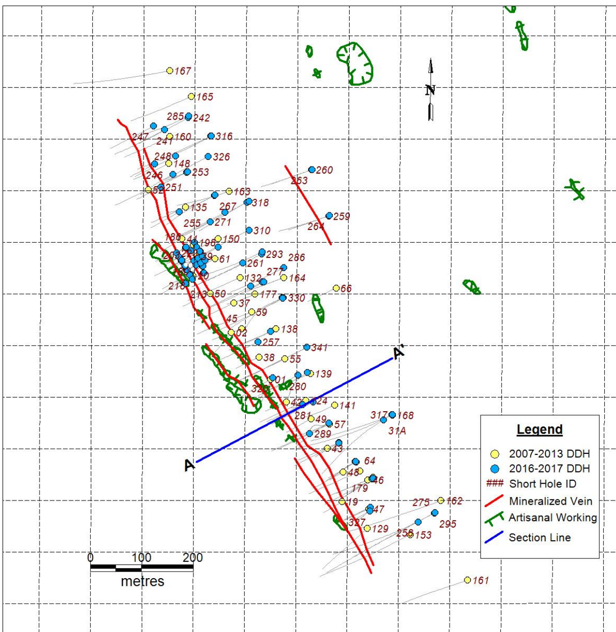
Figure 10.2: Plan Map – Serra Vein
