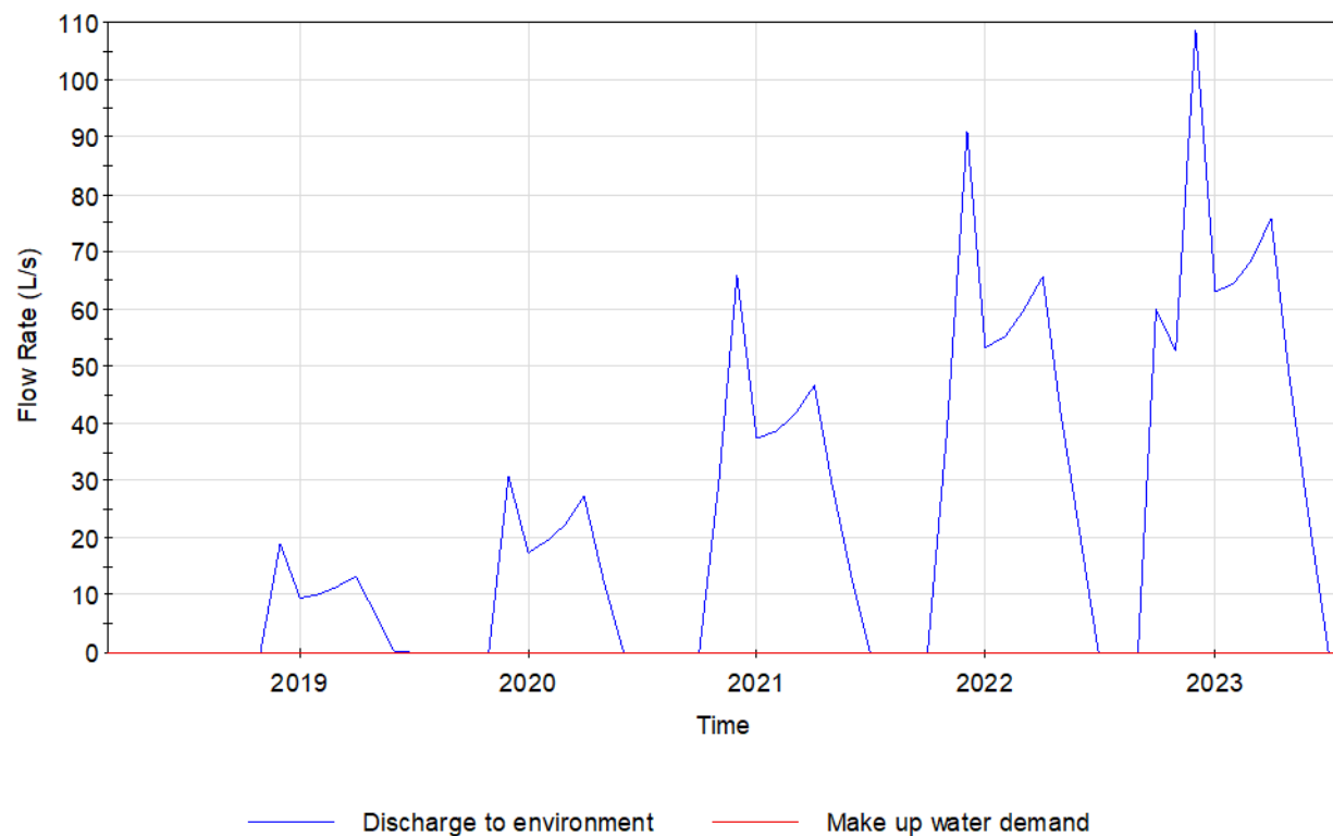
Figure 18.17: Discharge to the Environment & Makeup Water Requirements – 85 th Percentile
