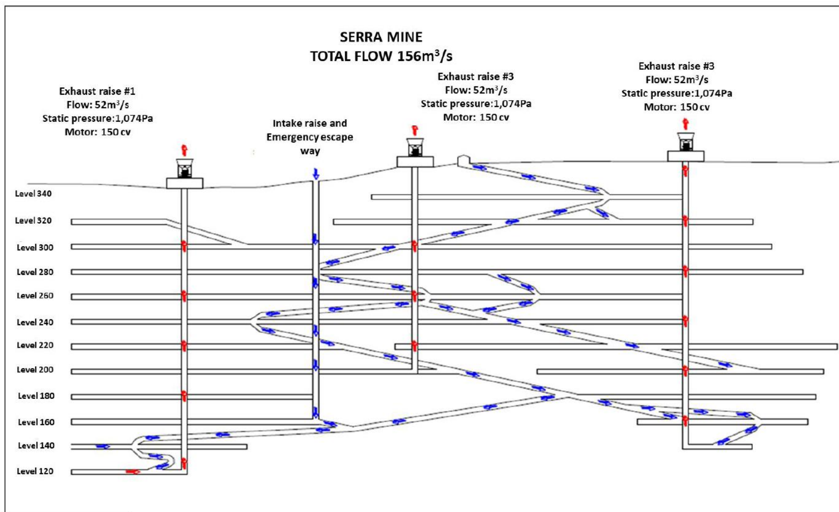
Figure 16.13: Airflow Paths - Serra
