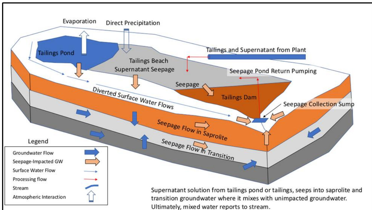
Figure 18.20: Conceptual Model
