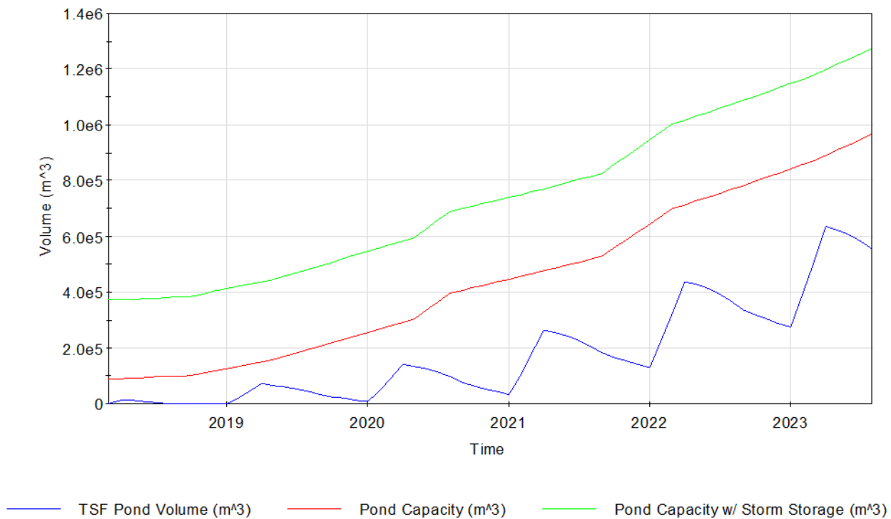
Figure 18.14: TSF Pond Storage – 23 rd Percentile
