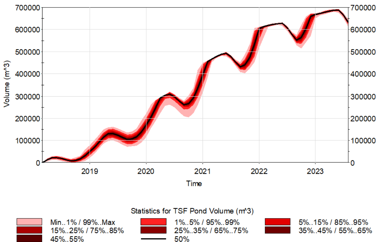
Figure 18.11: TSF Pond Storage
