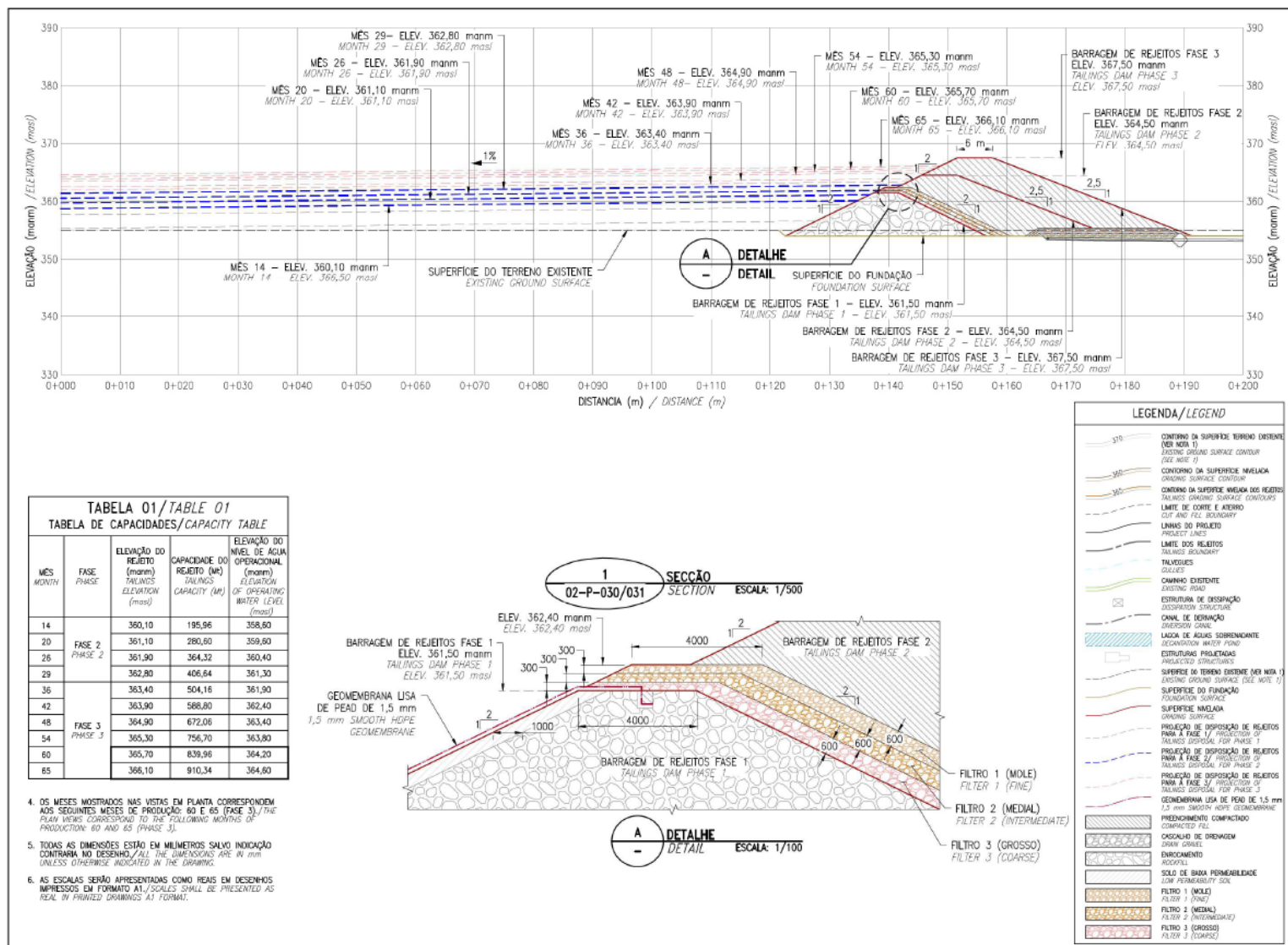
Figure 18.5: TSF Section
