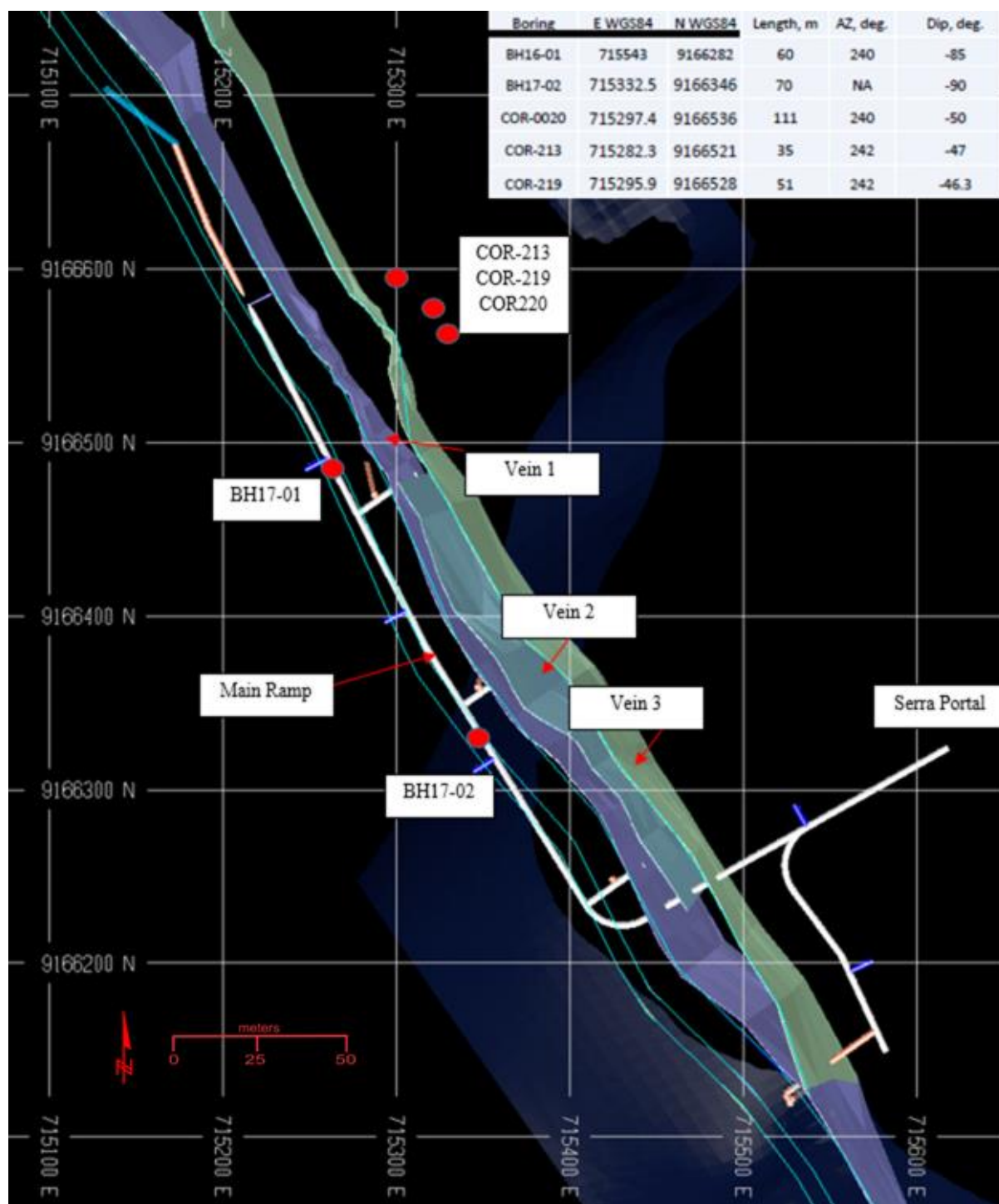
Figure 16.5: Serra Geotechnical Drill Hole Collars
