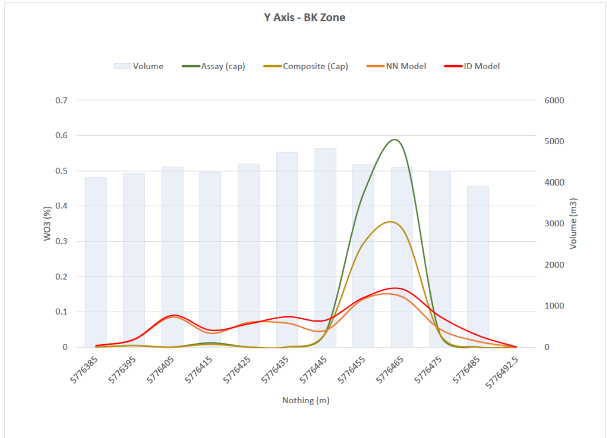
FIGURE 14-18: Y AXIS SWATH PLOTS (INDICATED AND INFERRED CLASSIFICATION)
