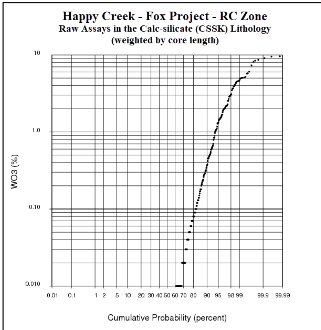
FIGURE 14-2: RAW ASSAY FREQUENCY DISTRIBUTION, RC ZONE IN CSSK LITHOLOGY
