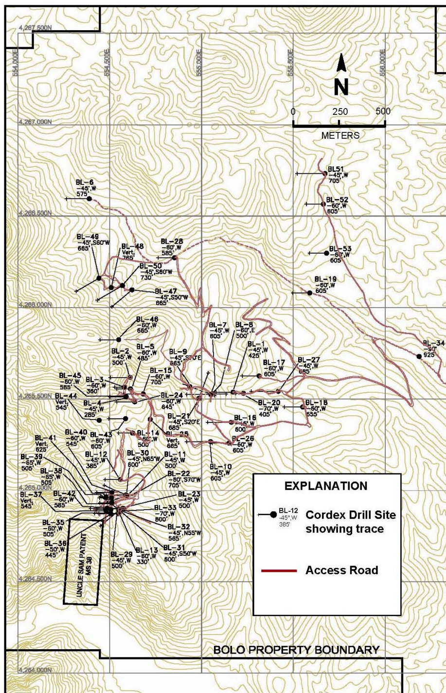
Figure 10.1 Columbus Gold Drill Hole Location Map, through 2013. Map from Columbus Gold (2013).
