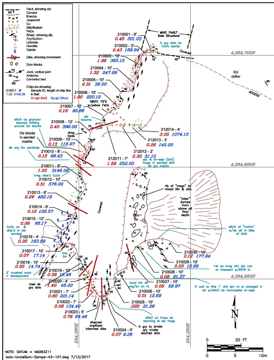
Figure 9.6. Gold (gpt) and Silver (gpt) in rock chip samples on the Uncle Sam Patent at Bolo. Map from Columbus Gold (2017).
