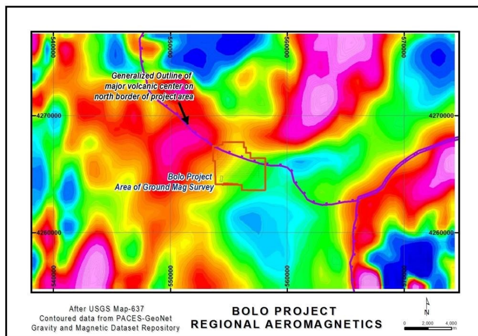
Figure 9.11 Regional Magnetics (RTP). Map from Columbus Gold (Modified after USGS Map 637 (USGS, 1968)).
