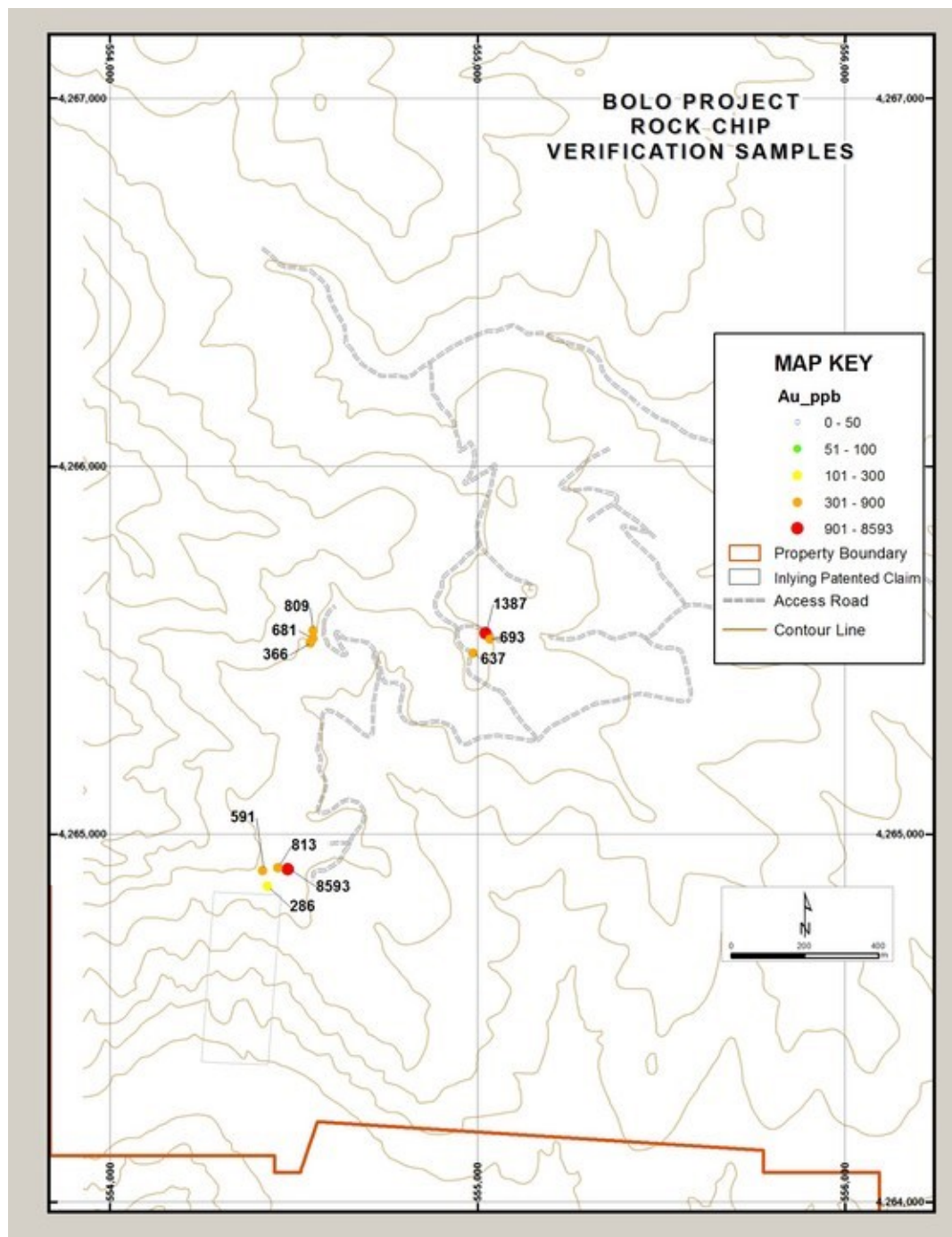
Figure 12.1 Gold (ppb Au) in Author's Verification Samples, 2012 sampling.
