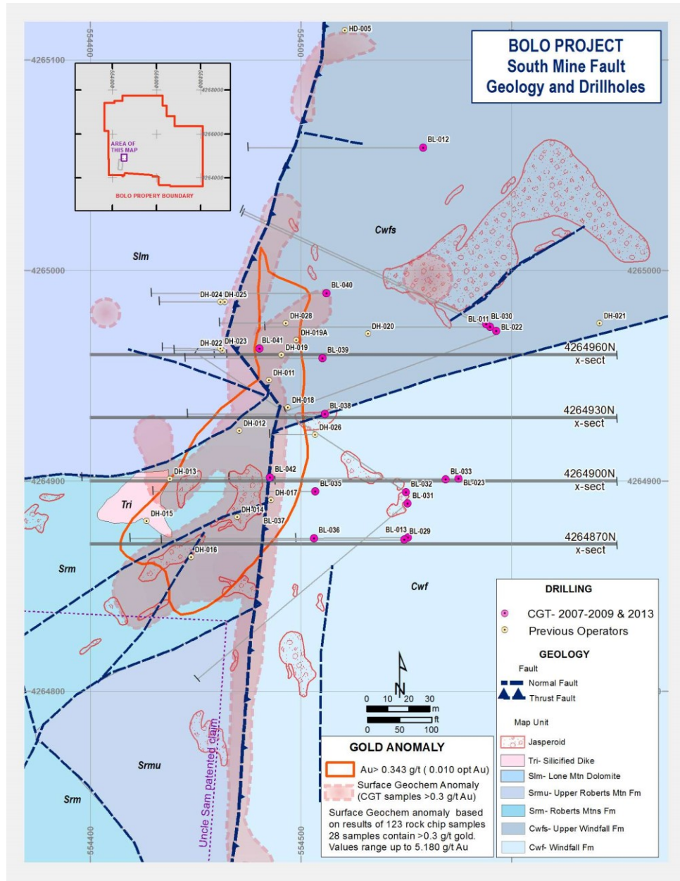
Figure 7.4 South Mine Fault Zone. Plan Map of Drilling (shows location of cross-sections in Figures 7.5, 7.6, 7.7 and 7.8). Map from Columbus Gold (2013).
