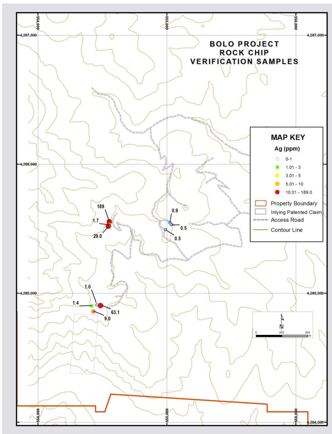
Figure 12.2 Silver (ppm Ag) in Author's Verification samples, 2012 sampling. Map from Columbus Gold (2013).
