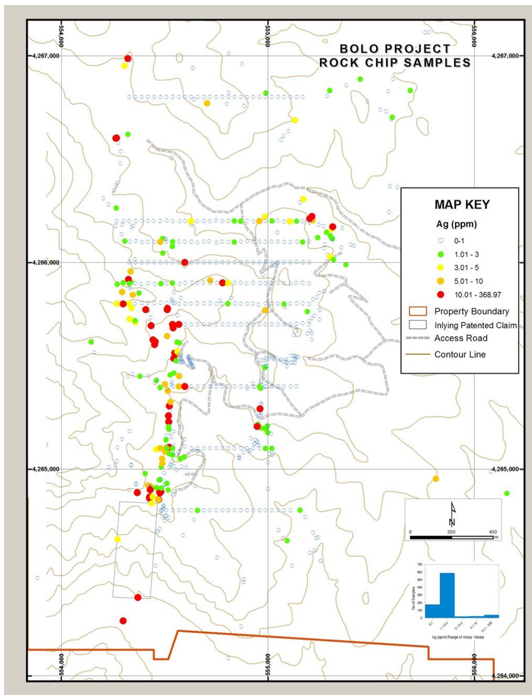
Figure 9.2 Silver in rock chip samples (ppm) on the unpatented claims at Bolo. Map from Columbus Gold (2012).
