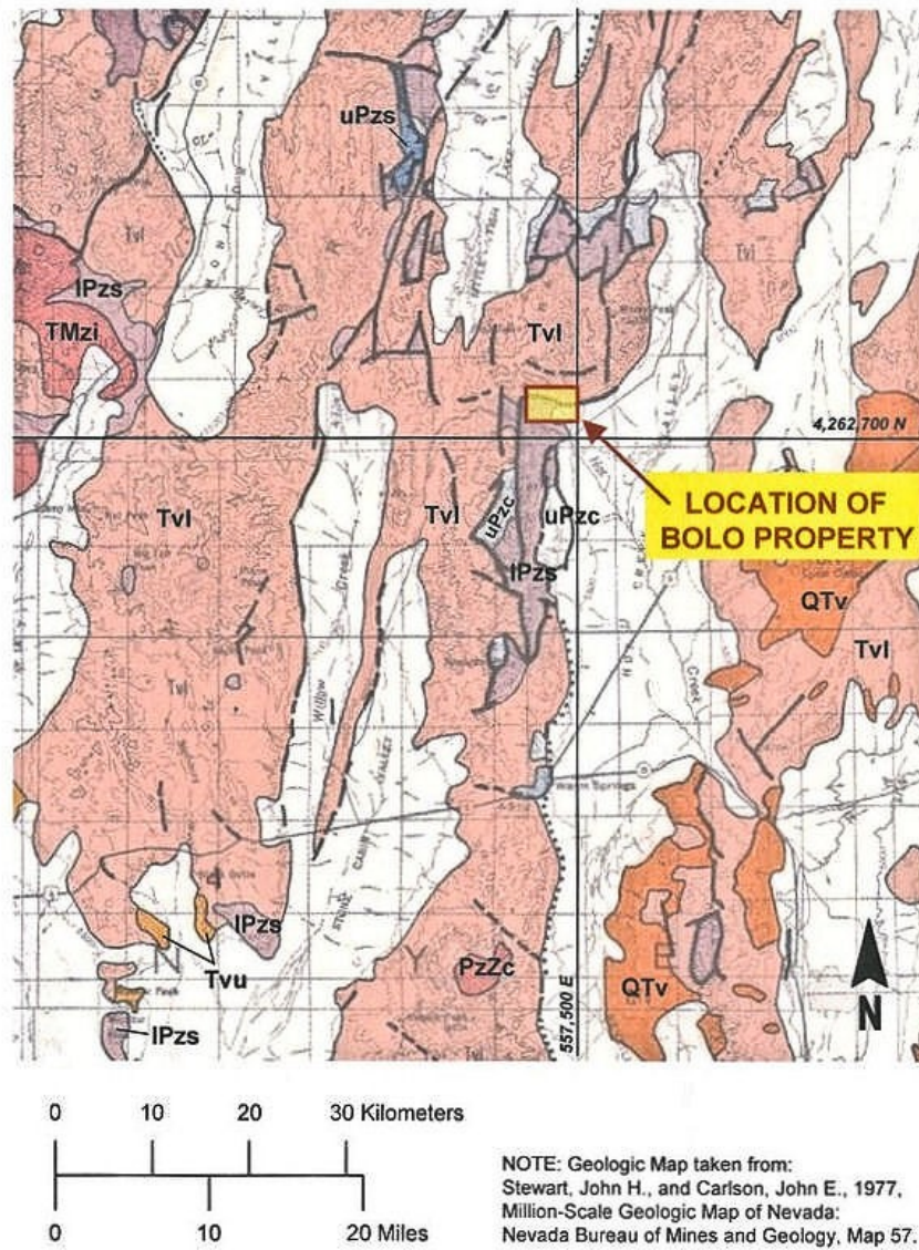
Figure 7.1 Regional Geologic Map. (Stewart and Carlson, 1977)
