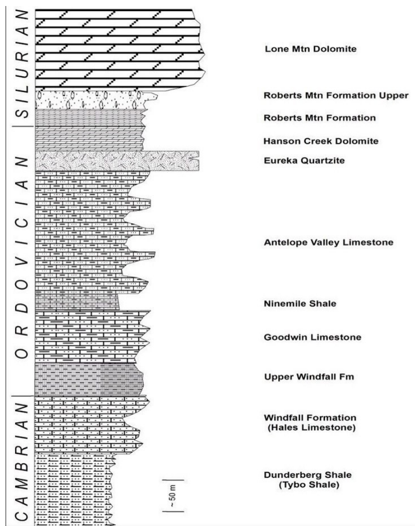
Figure 7.3 Generalized Paleozoic Stratigraphic Column, Bolo Property. From Columbus Gold (2011).
