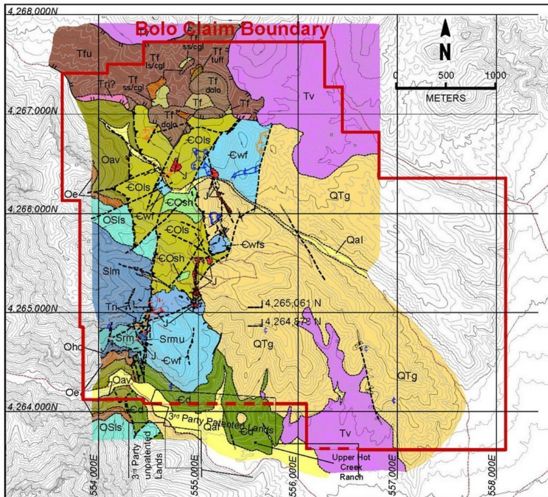
Figure 7.2 Geologic Map of the Bolo Property. Explanation on next page. Map from Columbus Gold (2011).
