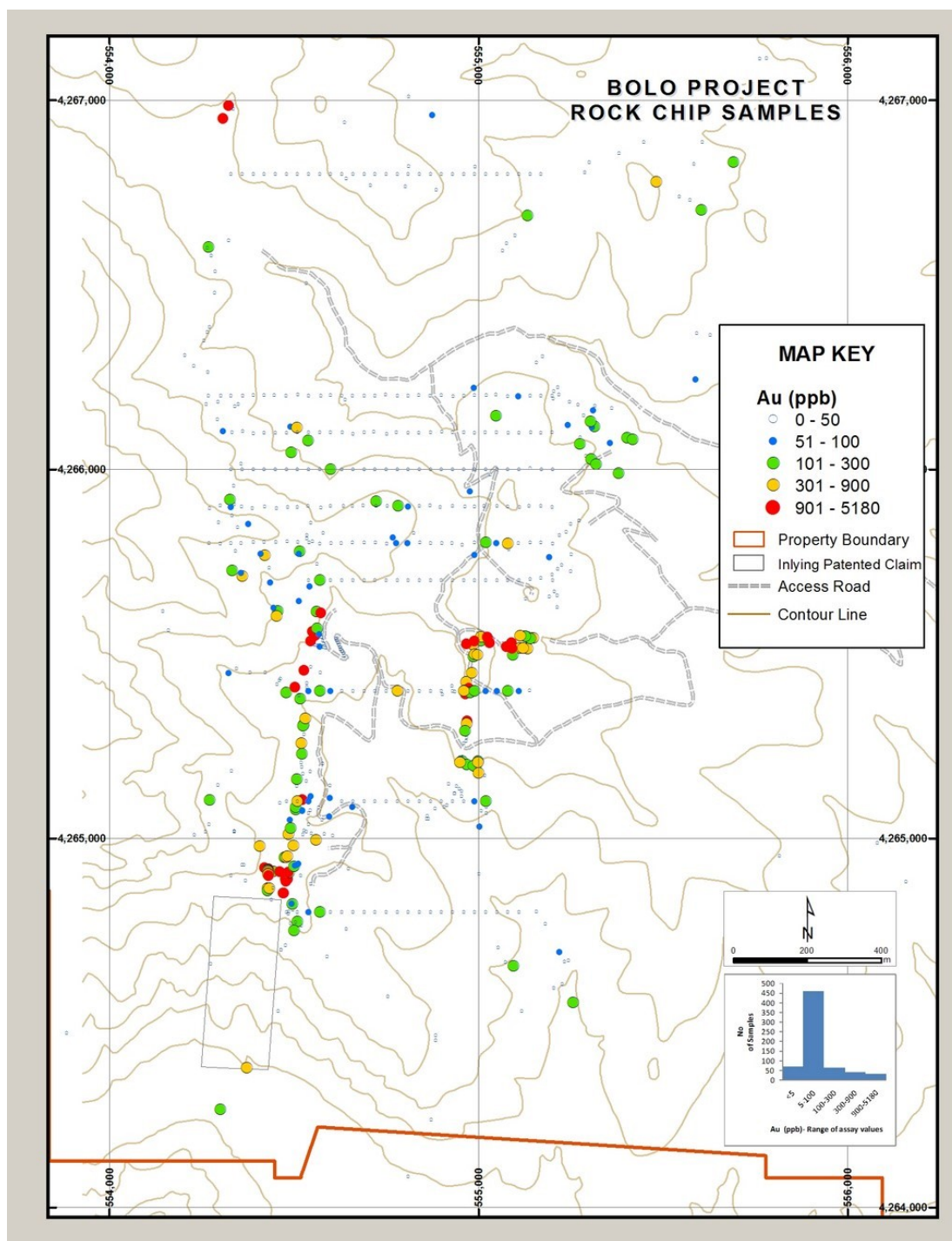
Figure 9.1 Gold in rock chip samples (ppb) on the unpatented claims at Bolo. Map from Columbus Gold (2012).
