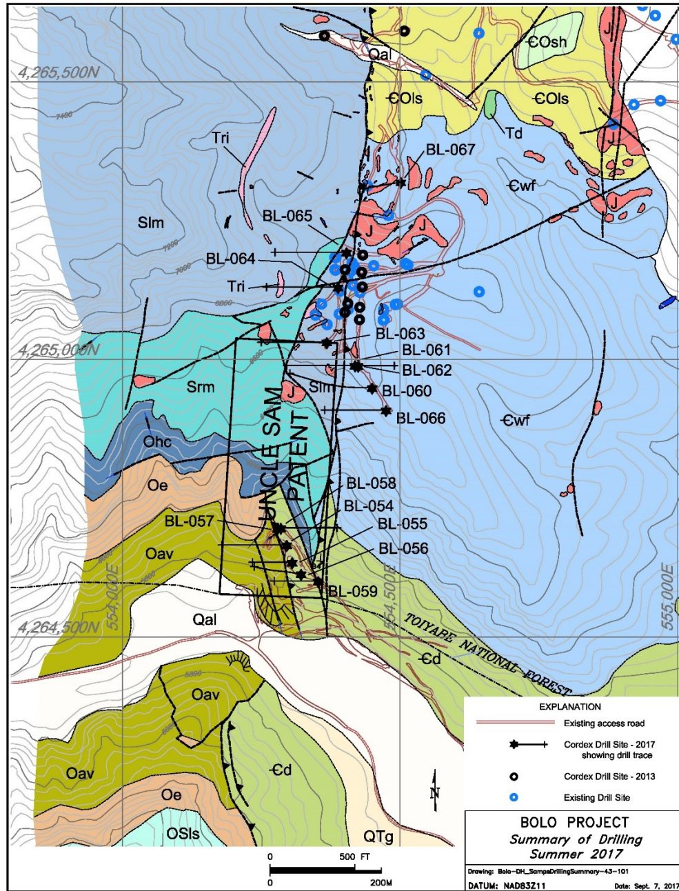
Figure 10.2 Columbus Gold Drill Hole Location Map; 2017 Drill Program. Map from Columbus Gold (2017).
