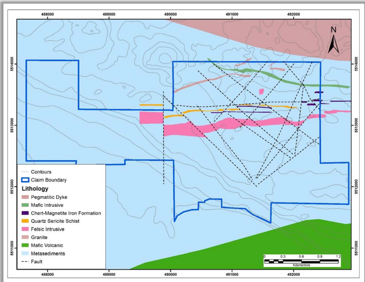
Figure 7.2 Property Geology
