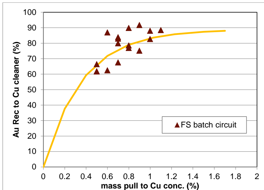
Figure 13-26: Cu cleaning circuit Au recovery vs mass pull to Cu concentrate
