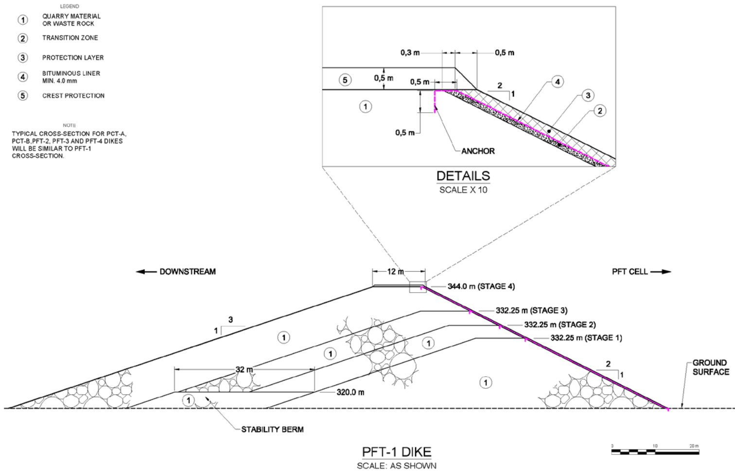
Figure 20-15: PFT-1 cross-section
