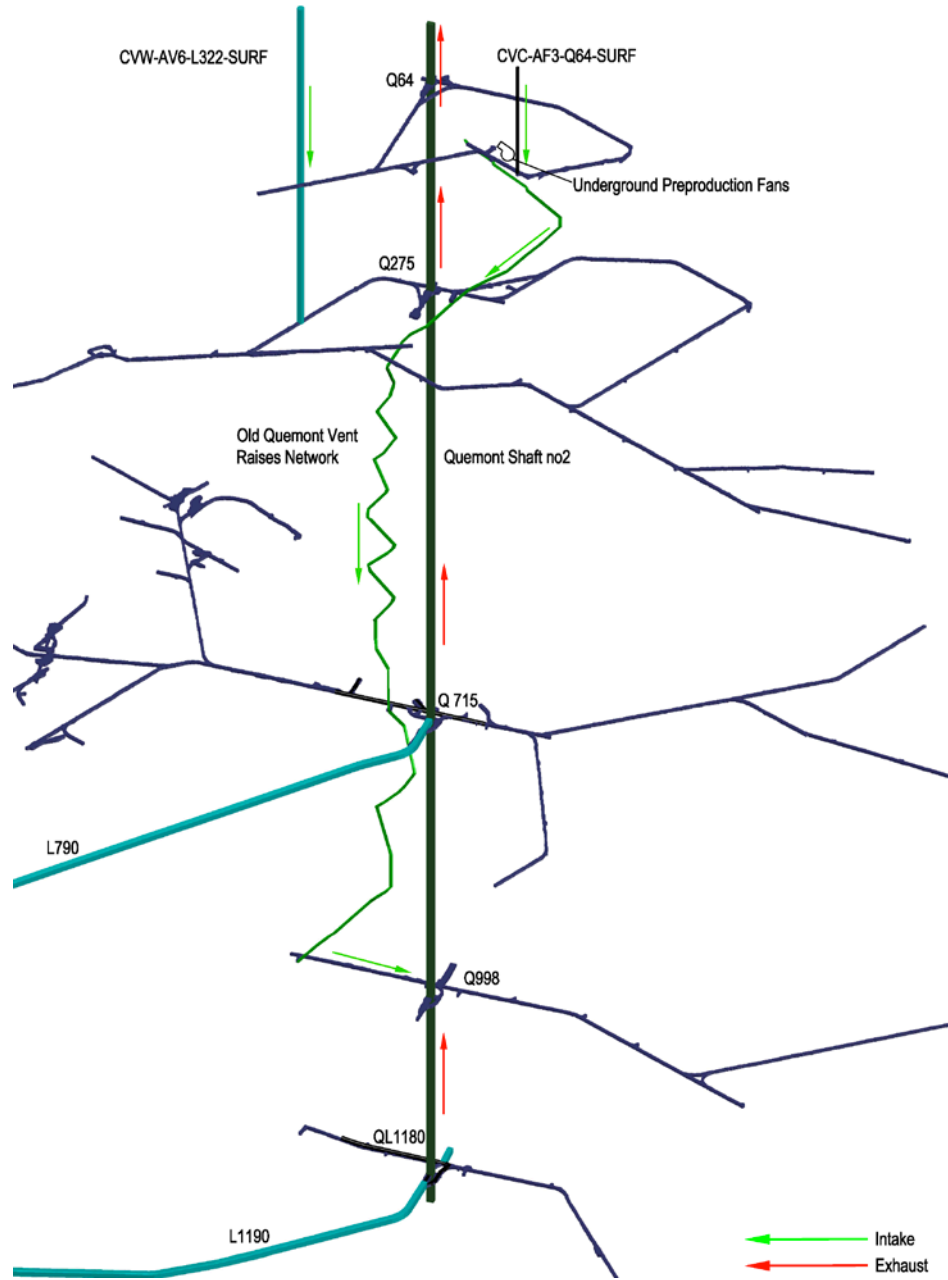
Figure 16-35: Complete preproduction/development ventilation network
