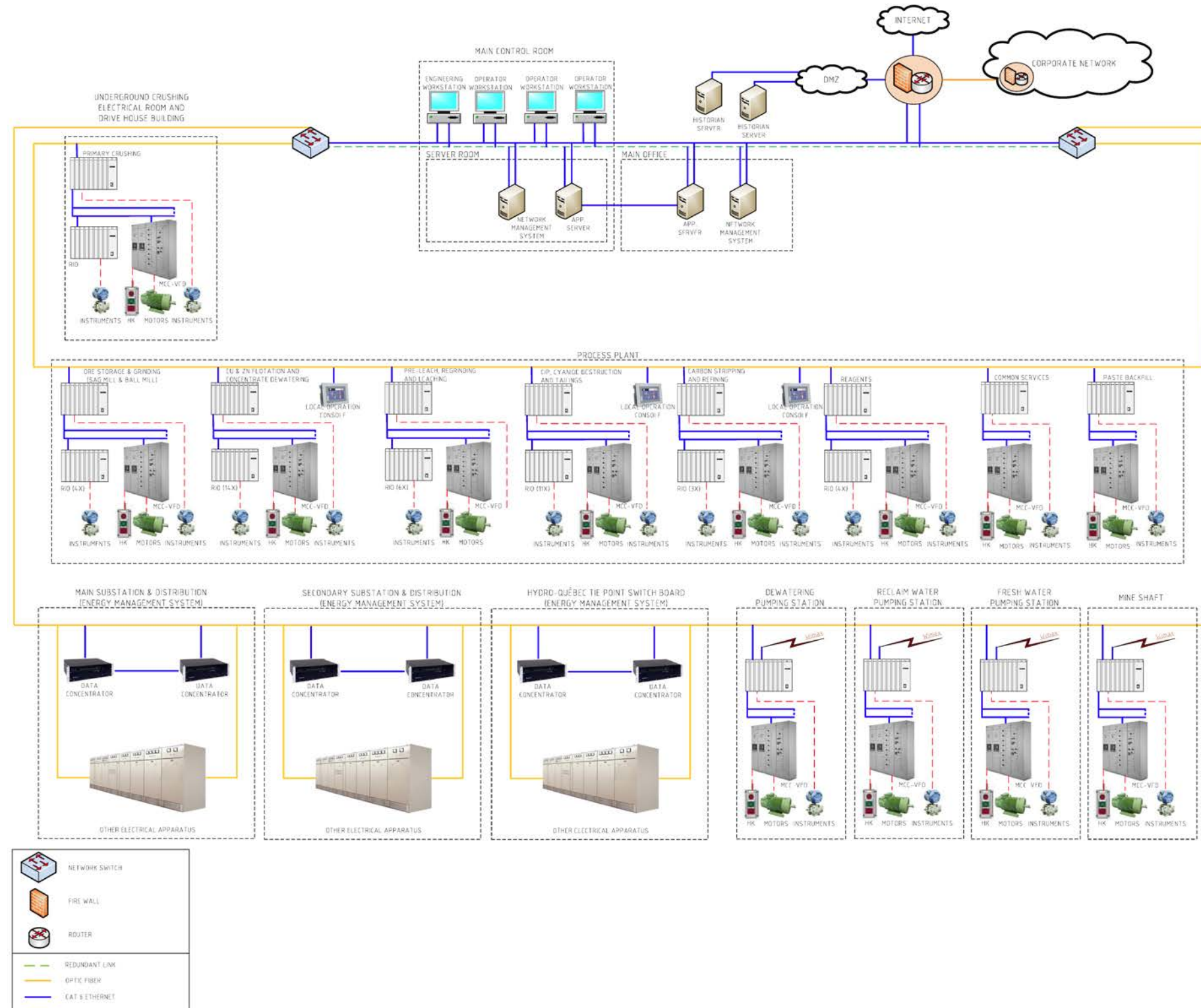
Figure 17-15: Proces plant control system generic topology
