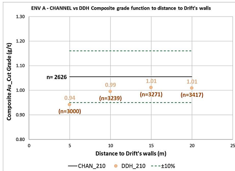
Figure 12-11: Comparison between channel sample composites and drill hole sample composites for ENV_A (Rock code 210) The contact plot (top) shows that drill hole composite grades are slightly lower than channel composite grades. A similar trend is observed when the comparison is made using distance from the wall of a sampled drift (bottom).
