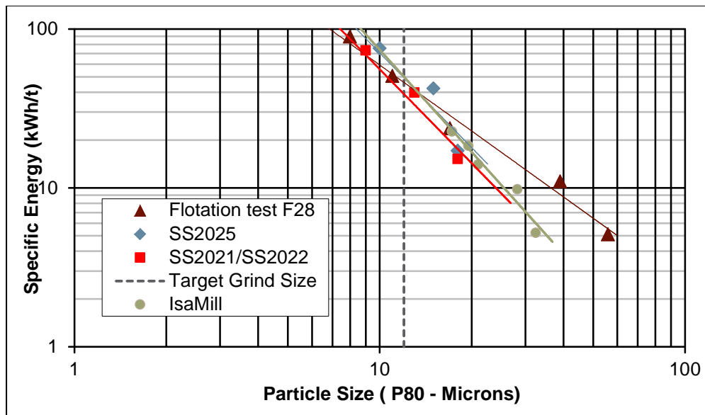
Figure 13-50: Comparison of HIG mill vs Isa mill signature curves
