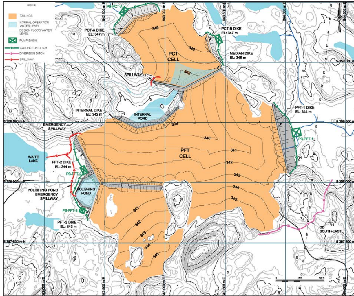
Figure 20-14: Surface TMF development sequence – Stage 5
