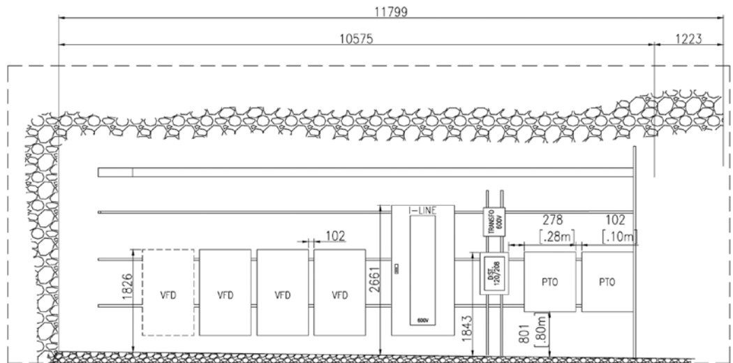
Figure 16-22: Typical production substation
