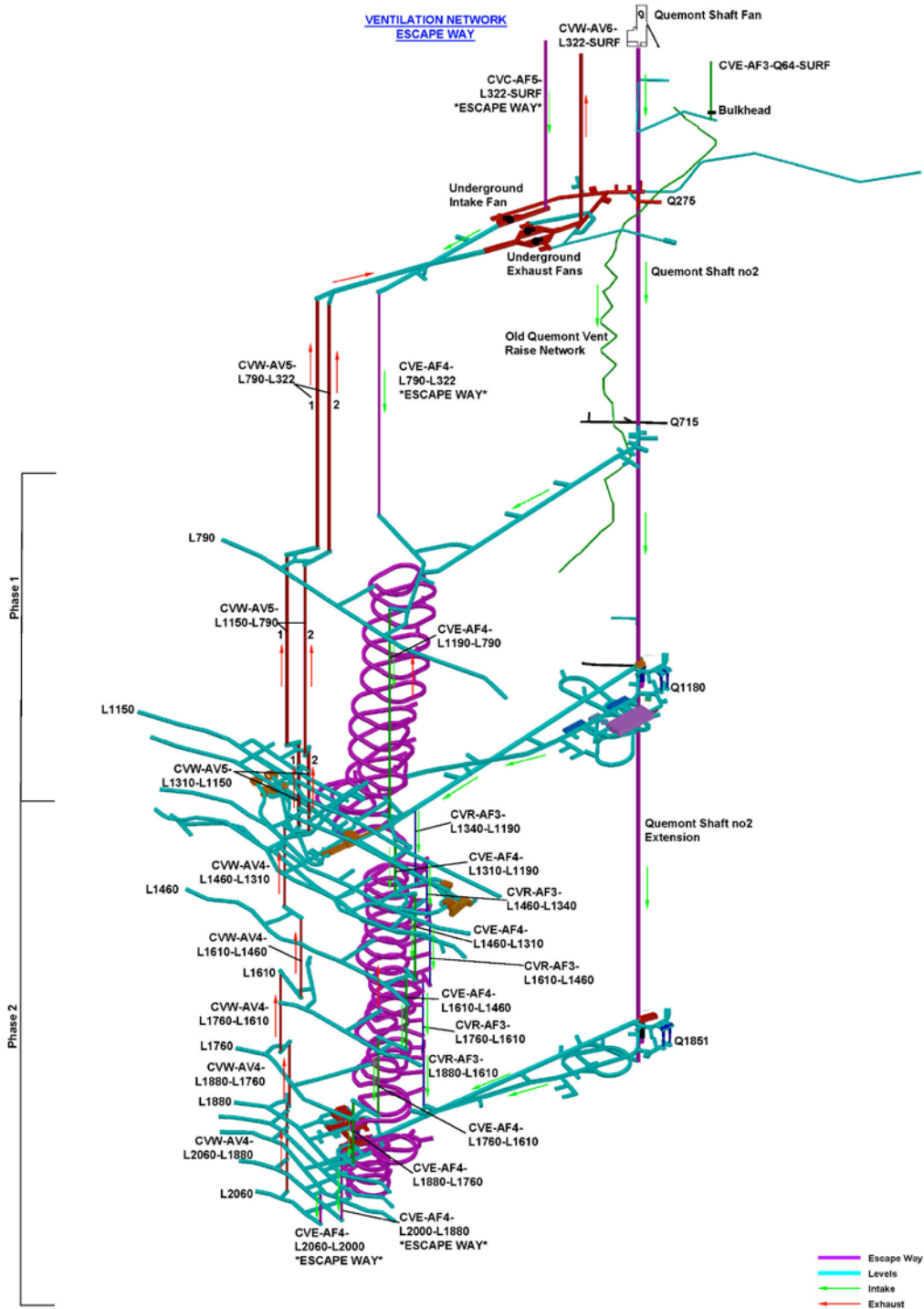
Figure 16-36: Permanent ventilation network with escape ways
