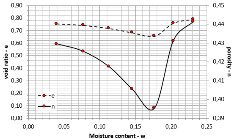
Figure 20-8b: PFT standard Proctor testing results
