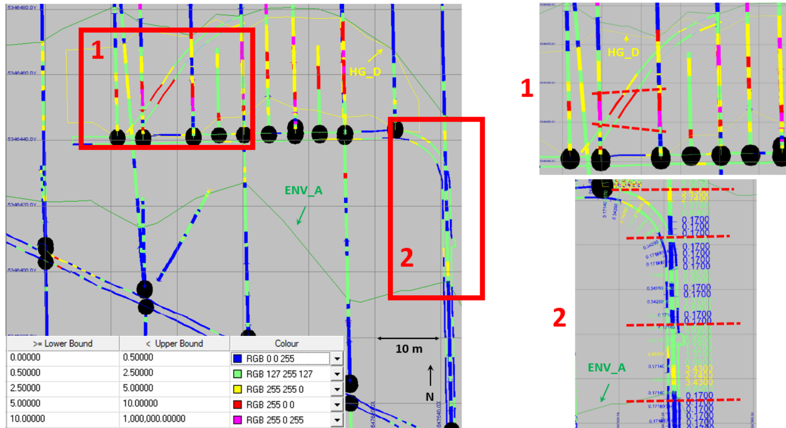
Figure 9-4: Plan view looking down on level 49 illustrating the relationship between gold grades in channel samples and those of nearby DDH (left) Close-up view #1 (top right) illustrates the correlation of high-grade gold values in the HG_D mineralized zone. Close-up view #2 (bottom right) illustrates the correlation of low-grade gold values in the ENV_A mineralized zone. Red dashed lines indicate correlations
