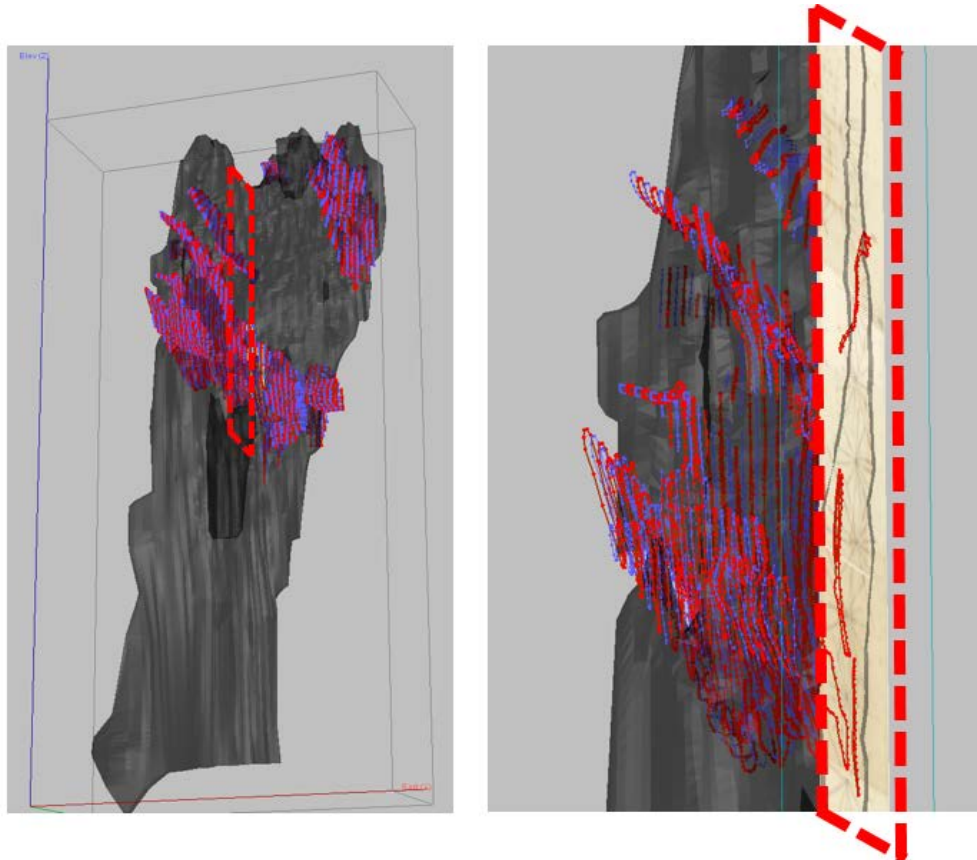
Figure 9-8: 3D views of digitized lines used to form “Dyke M” domains Relevant domains were digitized in the middle and upper portions of the Horne 5 deposit (right) according to historical information, which includes Noranda’s interpreted geology on vertical cross sections and the geology along drill holes (left)
