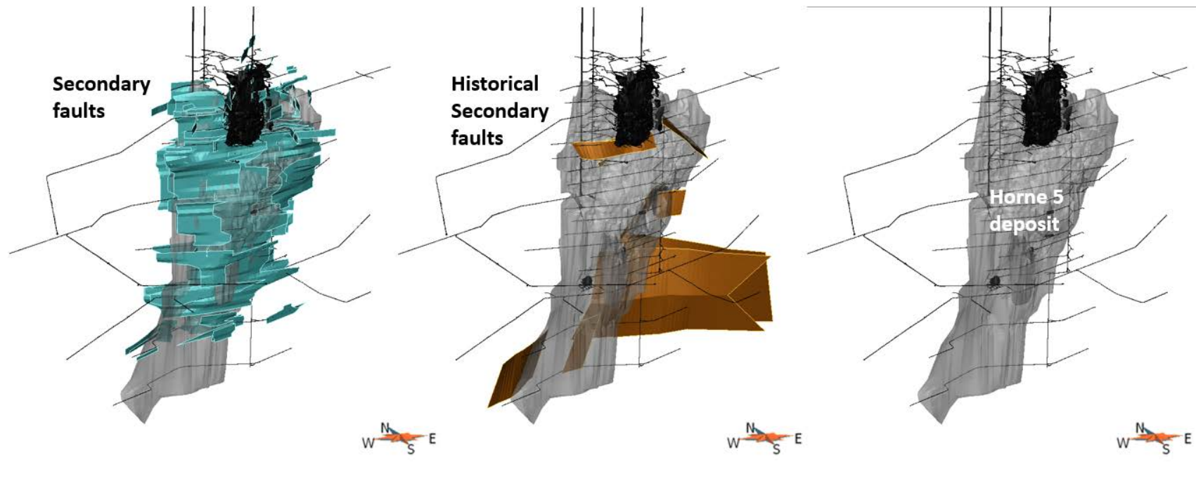
Figure 7-29: 3D view of updated 2016 Horne 5 lithostructural model for secondary faults More than 100 individual panels have been modelled based on DDH and underground mapping information (left). Historical secondary faults, from De Kemp works mainly, have been also used (centre). The Horne 5 deposit ENV_A model is shown for illustrative purposes (right).
