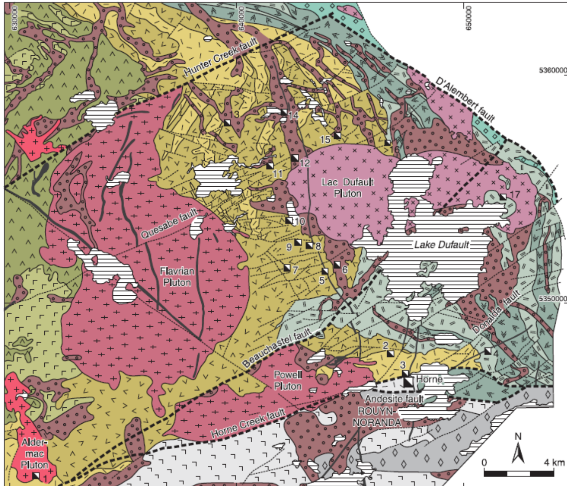
Volcanic-hosted massive sulphide deposits: 1 = Aldermac, 2 = Joliet, 3 = Quemont, 4 = Delbridge, 5 = D68, 6 = Millenbach, 7 = Corbet, 8 = Amulet A, 9 = Amulet C, 10 = Amulet F, 11 = Old Waite, 12 = East Waite, 13 = Ansil, 14 = Vauze, 15 = Norbec, 16 = Newbec, and 17 = Gallen
