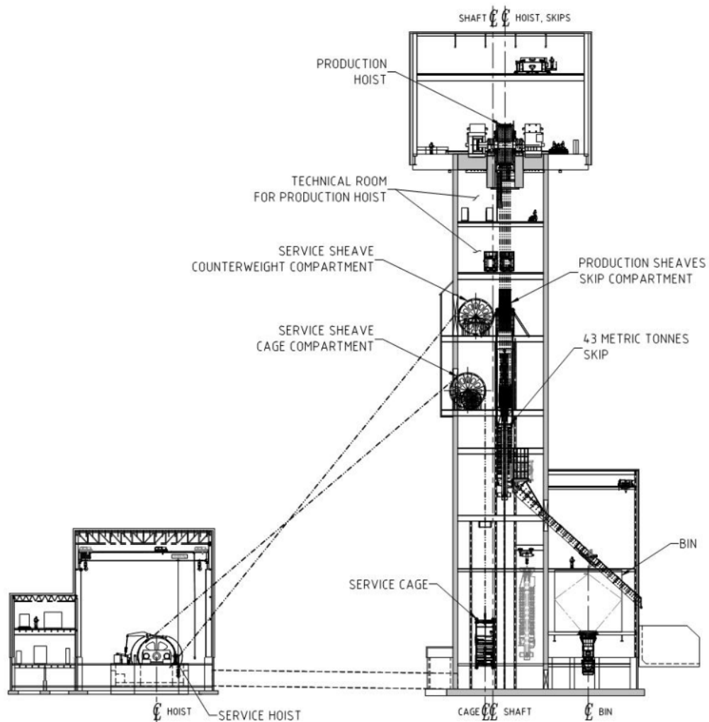
Figure 18-8: Hoisting system
