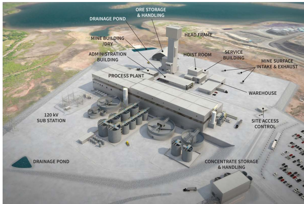
Figure 1-4: General site layout – Horne 5 Mining Complex
