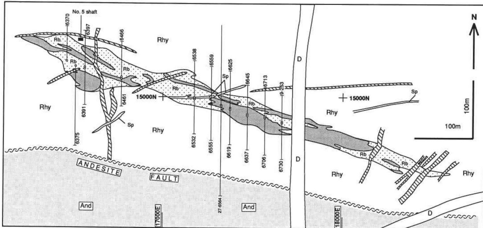
The Horne 5 deposit (light stipple) consists of a tabular series of intercalated zones of disseminated sulphides with lenses of pyritic massive sulphides (shaded), all broadly concordant with east-southeast-striking rhyolitic units. See legend of Figure 7-7. R= rhyolite; Rb= rhyolite breccia, Rt= rhyolite tuft Rc= chloritic rhyolite; Rs= sericitized rhyolite; stippled, massive sulphides; Sp= syenite porphyry; hachured= metadiabase dike; D= younger diabase dike; And= Andesite; Sh= shear zone. Drill holes used in the study by Barrett et al. (1991) are shown. Galleries were omitted for clarity. (From Barrett et al., 1991)
