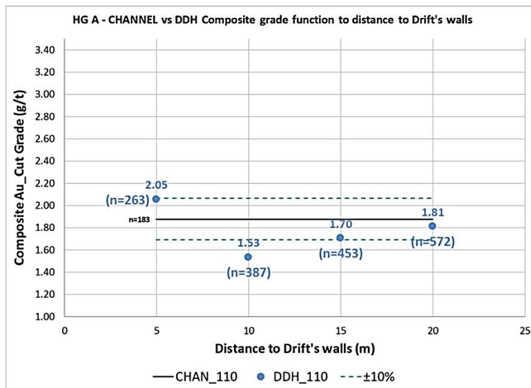
Figure 12-12: Comparison between channel sample composites and drill hole sample composites for HG_A (Rock code 110)
