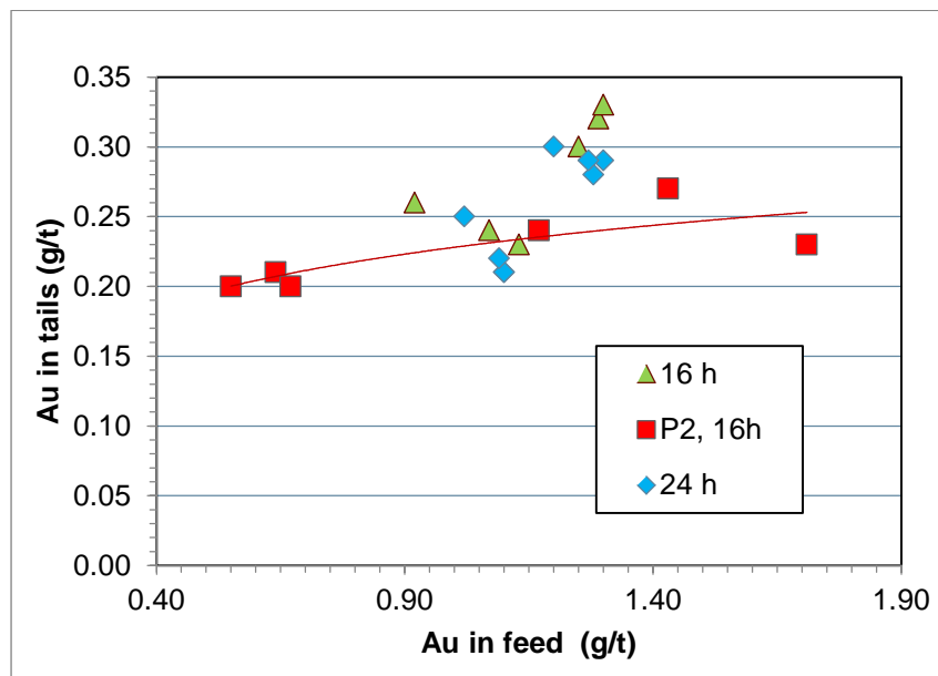
Figure 13-45: Au in pyrite conc. cyanidation tails vs Au in feed to circuit
