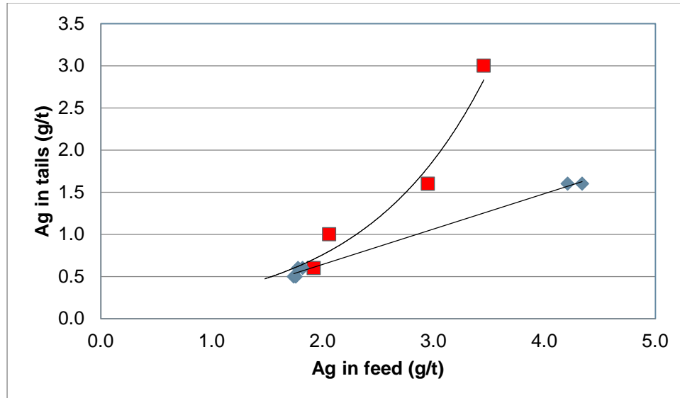
Figure 13-48: Ag in pyrite tails leaching tails vs Ag in feed to circuit
